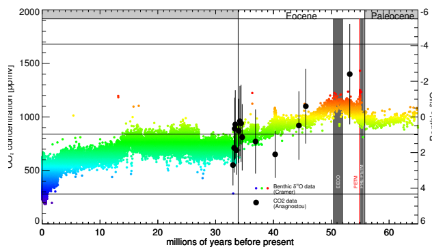
Figure 5. Atmospheric CO 2 as derived from boron isotopes in the Eocene by (Anagnostou et al., 2016) (black circles and error estimates). Horizontal lines show 280 ppmv (typical preindustrial value), and 840ppmv and 1680 ppmv, corresponding to the deepmip-stand-3 ×CO 2 and deepmip-stand-6 ×CO 2 simulations. Also shown are the DeepMIP palaeo intervals - EECO (grey shaded region), pre-PETM (grey shaded region), and the PETM (vertical red line), and the climate evolution over the last 65 million years, as expressed by the benthic oxygen isotope record of Cramer et al. (2009) (coloured dots). Note that the formal definition of the start and end date of each time period is still to be finalised.
