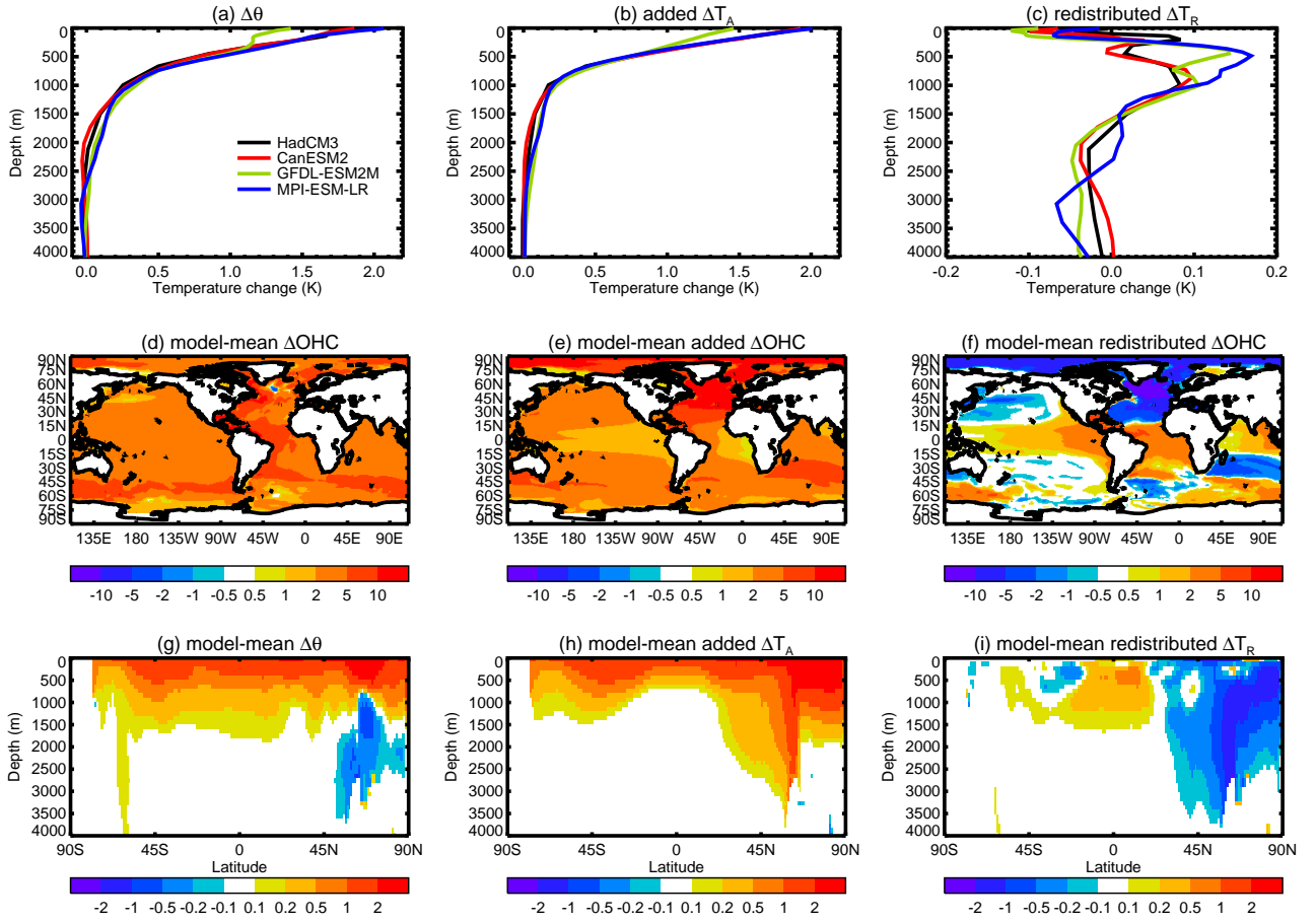
New version of Fig. 9. Change in ocean temperature \theta (left) and tracers of added heat (centre) and redistributed heat (right) in the final decade of the faf-heat experiment, (top) global-mean change in tracer (K) as a function of depth, with different scales for the temperature axis, (middle) model-mean change in heat content ( \text{GJ m}^{-2} , the vertical integral of the change in tracer multiplied by volumetric heat capacity), (bottom) model-mean zonal-mean cross-sections of the change in tracer (K). We will note that (a,d,g) repeat earlier figures, and give their numbers, which will have changed from the submitted manuscript because of reordering Sect. 3. This figure will be in landscape format.
