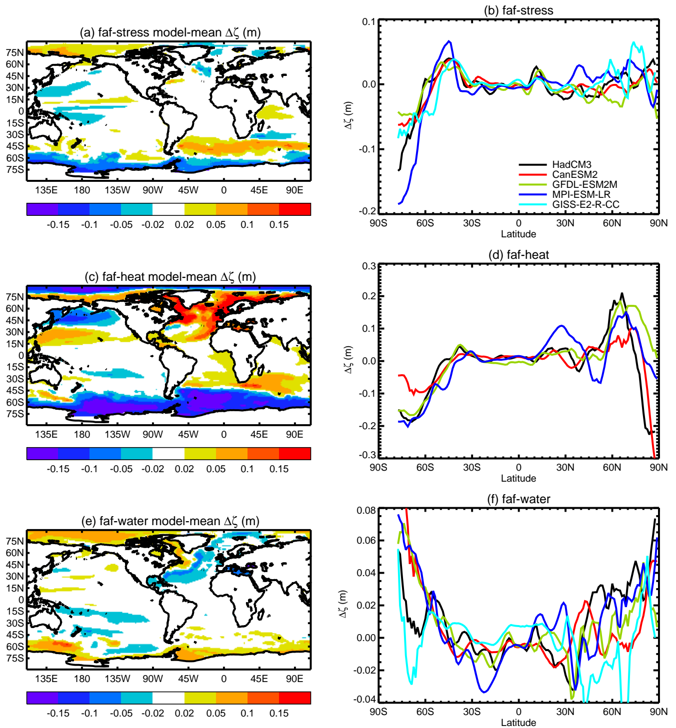
Figure 8. Change in dynamic sea-level \Delta\zeta (m) in the time-mean of the final decade of the FAFMIP experiments relative to the control, model mean on the left, zonal means of individual models on the right. Note that the panels on the right have different scales for the \Delta\zeta axis.
