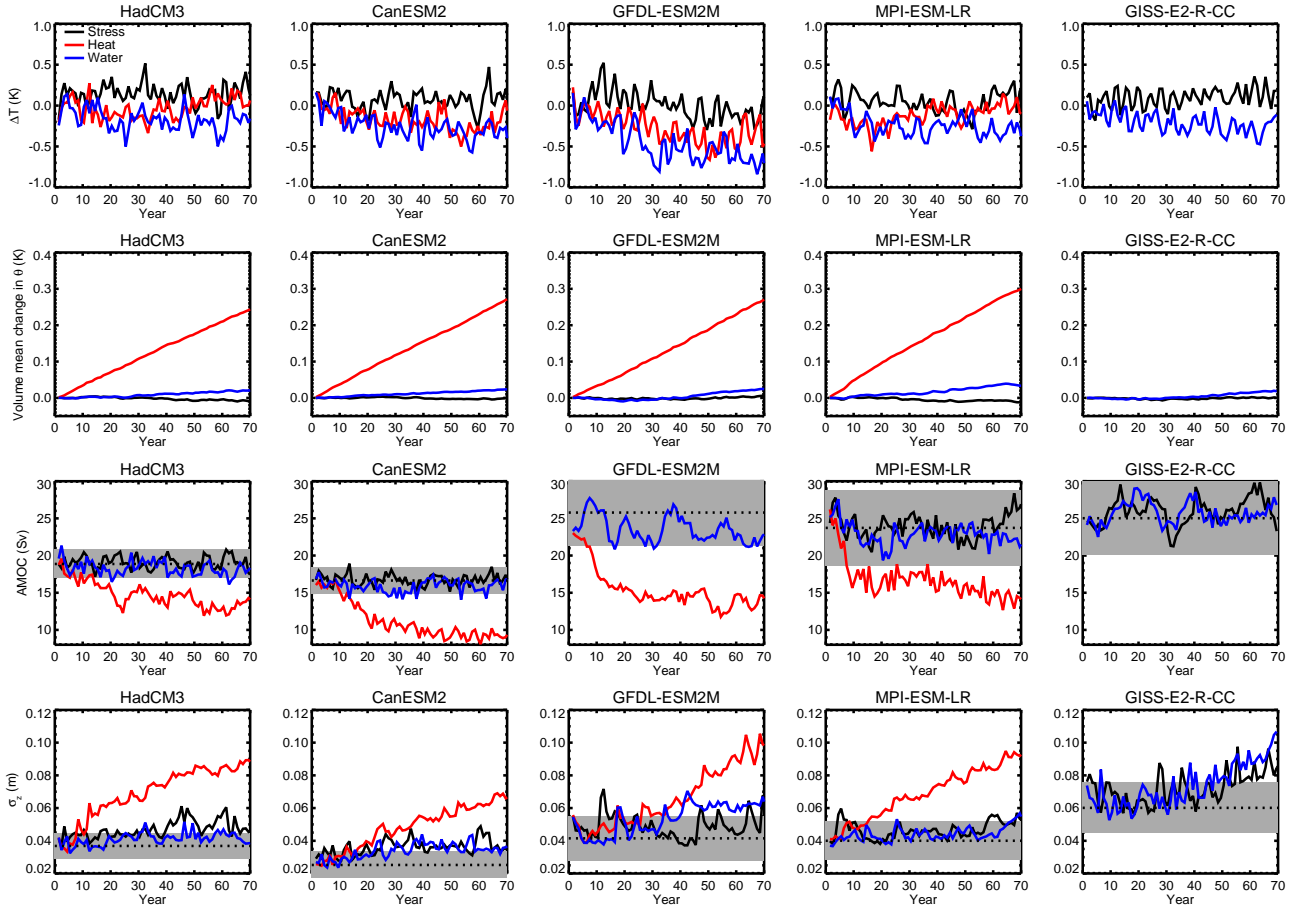
New version of Fig. 4. Annual timeseries in faf-stress, faf-heat and faf-water, according to the key in the first panel. Top row, global-mean surface air temperature change (K) with respect to the control time-mean; second row, ocean volume-mean temperature change (K) with respect to the corresponding year of the control; third row, maximum of the Atlantic meridional overturning streamfunction (Sv); bottom row: \sigma_\zeta (m), the spatial standard deviation of \Delta\zeta , the dynamic sea-level change relative to the 70-year time-mean in the control experiment. For the AMOC and \Delta\zeta , the grey band indicates the range of values which do not differ significantly (as defined in the text) from the control time-mean, which is indicated by the dotted line. This figure will be in landscape format.
