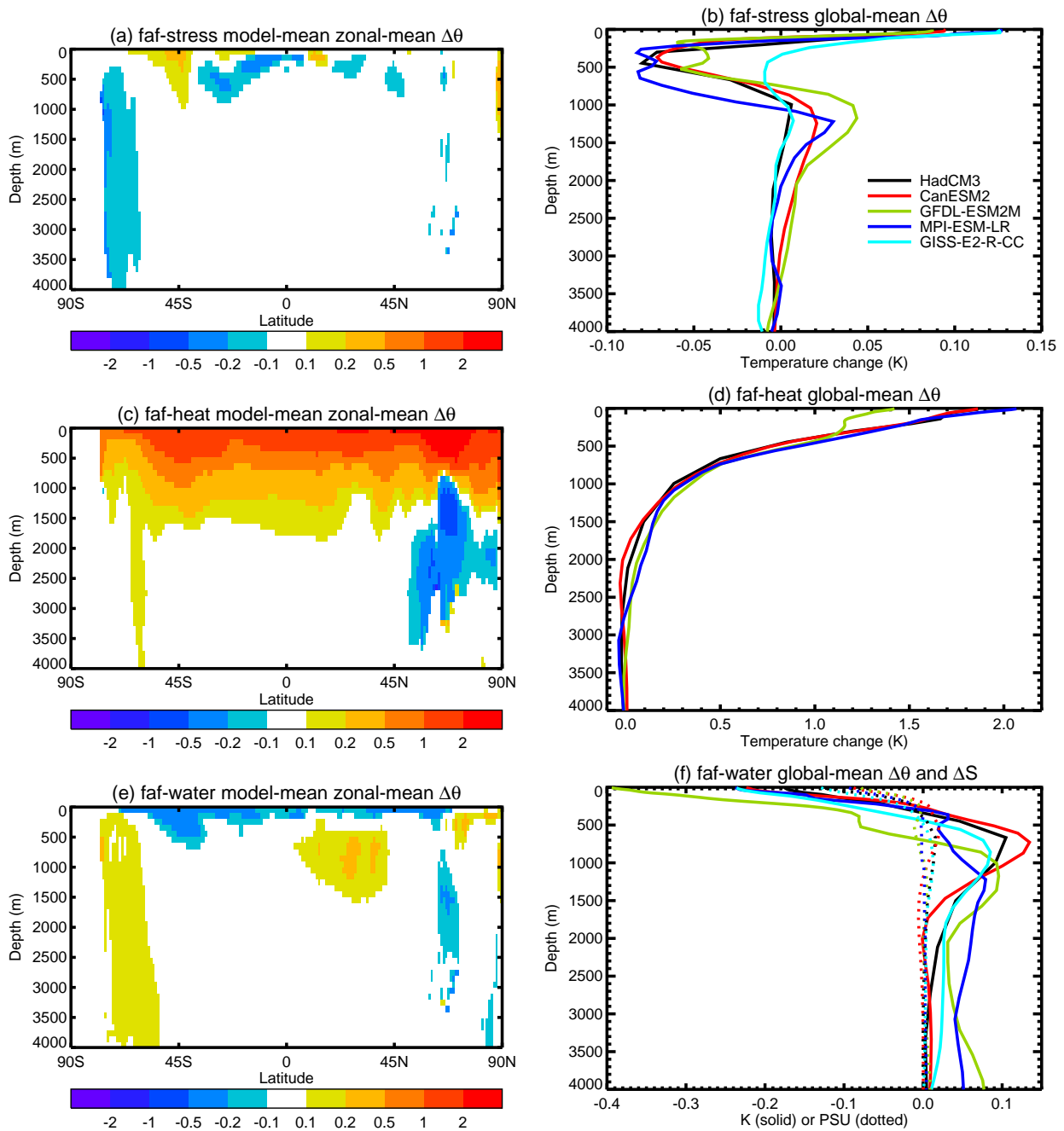
Figure 7. Model-mean change in ocean temperature \theta (K) in the time-mean of the final decade of the FAFMIP experiments relative to the control, model-mean zonal-mean cross-sections on the left, global means as a function of depth of individual models on the right. Note that the panels on the right have different scales for the temperature axis.
