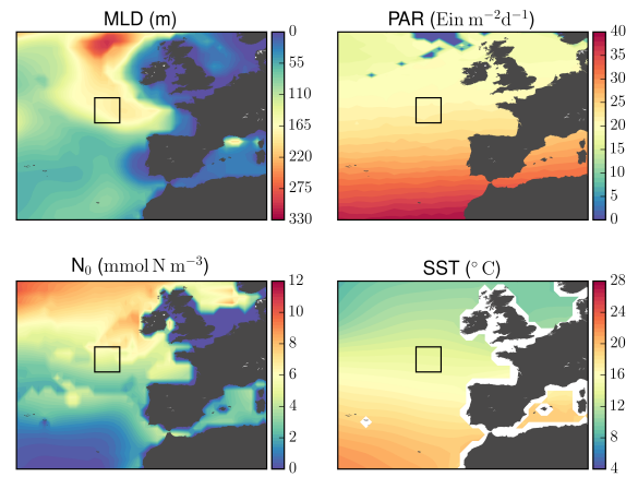
Figure 1. Environmental forcing variables considered in PhytoSFDM. The data shown are annual average of mixed-layer depth (MLD), photosynthetic active radiation (PAR), sea surface temperature (SST), and nitrogen concentration below the mixed-layer ( N_0 ). The square boxes mark the location of the test-case simulation.
