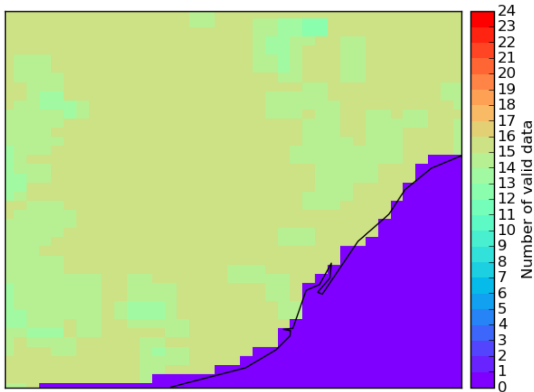
Supplementary figure 1. Number of valid MODIS data after quality control in each gridpoint, between May-September 2011, during night hours.
