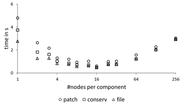
Figure 3. Performance—Time required for global search and calculation of YAC weights for 1st-order conservative remapping different interpolation methods in both directions between an ICONR2B06 grid and a 405x405-cubed-sphere grid
