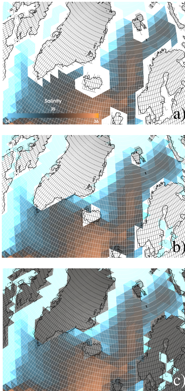
Figure 1. Interpolation of WOA09 January monthly mean sea surface salinity given on white rectangles interpolated to an ICON grid (triangles) using the YAC interpolation stack with 1st-order conservative remapping (a) plus 1st-order polynomial fit (b) plus fixed values (c). (for further details see Sec. 2.4)
