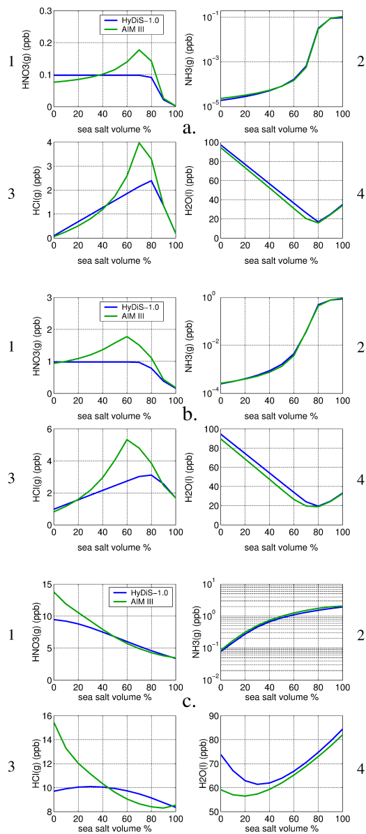
Figure 5: Box modelling evaluation of HyDiS-1.0 against AIM III with initial mixing ratios of \text{HNO}_3(\text{g}) and \text{NH}_3(\text{g}) of 0.1 (a), 1 (b) and 10 (c) ppb. The sea salt volume fraction is varied according to the values given in Table 1. The equilibrium vapour pressures are calculated with HyDiS-1.0 and AIM III for the equilibrium particle composition assessed with the former. The vapour pressures are given as mixing ratio equivalents for \text{HNO}_3 (1), \text{NH}_3 (2) and \text{HCl} (3) along with the total particle water mass (4). Note that particle composition is not size-dependent and that due to equilibrium composition discrepancies the AIM III \text{HCl} vapour pressure may be larger than its total amount.
