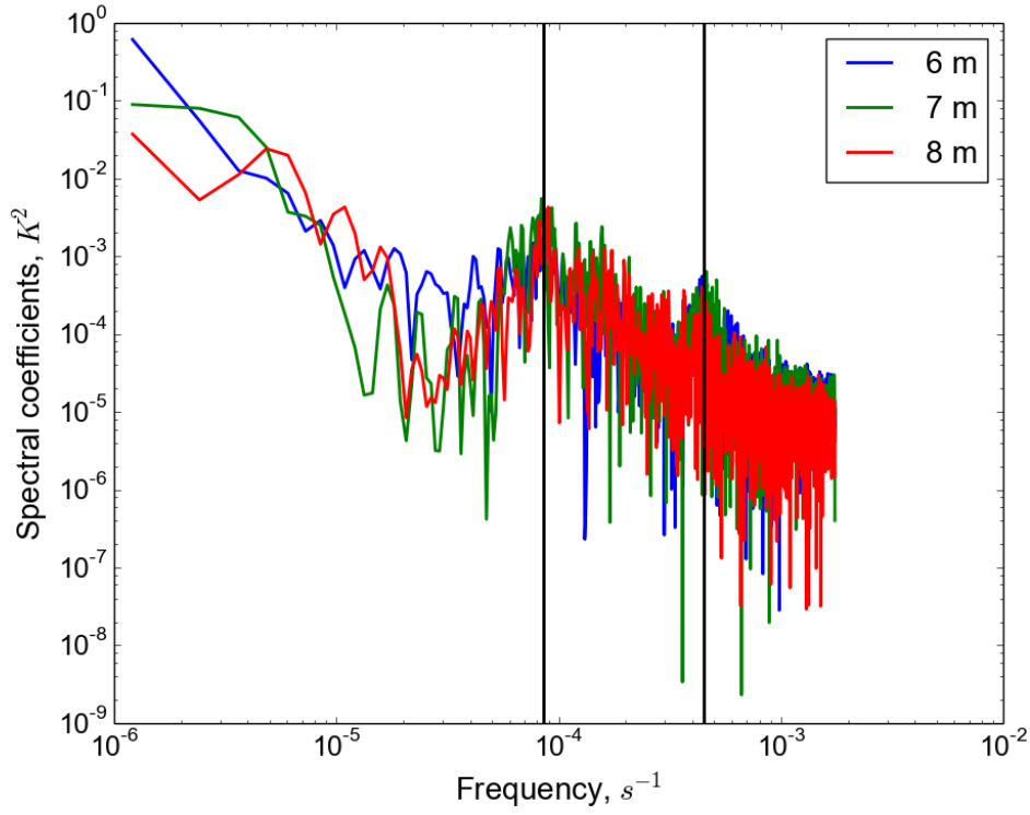
Figure 13: Fourier spectrum of water temperature fluctuations at depths 6 m, 7 m and 8 m. Two vertical lines point at maxima corresponding to \omega = 8.5 * 10^{-5} \text{ s}^{-1} ( T_{seiche} \approx 20.5 \text{ hour} ), left, and \omega = 4.5 * 10^{-4} \text{ s}^{-1} ( T_{seiche} \approx 3.9 \text{ hour} ), right
