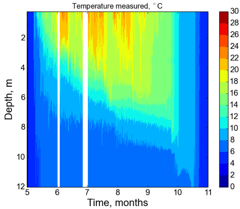
(b) Temperature, measured.
