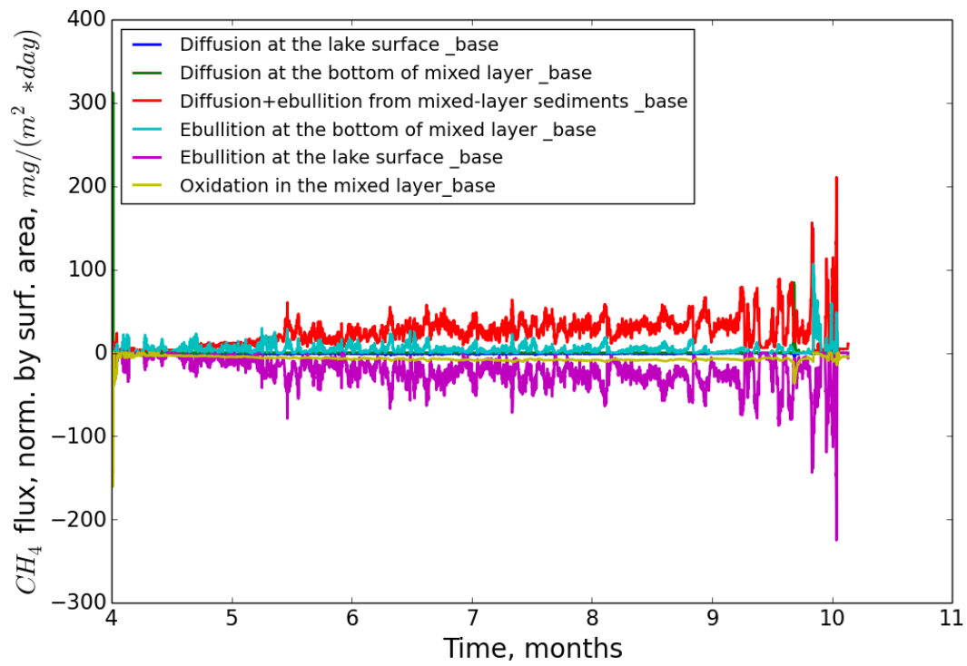
Figure 15: The components of \text{CH}_4 balance in the surface mixed layer, normalized by lake surface area. Positive terms increase \text{CH}_4 concentration in the mixed layer and negative ones are these decreasing \text{CH}_4 content. Suffix "_base" means baseline experiment
