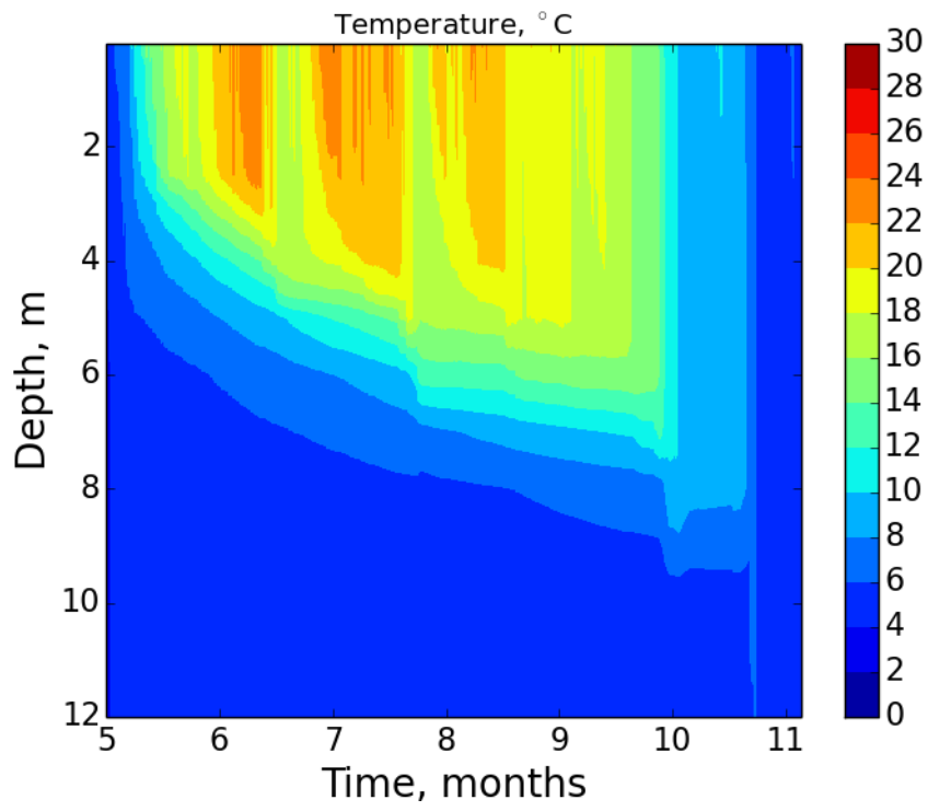
(a) Temperature, reference model run.
