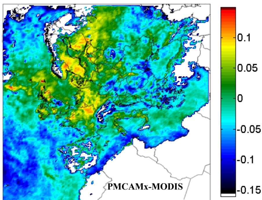
31 Figure 4. Difference of the PMCAMx from MODIS ( QAC \geq 1 ) monthly mean AODs during May 32 2008. Positive means that PMCAMx overpredicts AOD compared to MODIS. There were not enough 33 dust-screened AOD retrievals for the model evaluation in the white areas. 34 35 36 37 38
