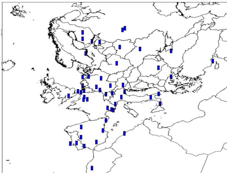
Figure 1. Geographical distribution of the 50 AERONET stations used in the present study.
