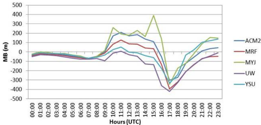
Figure 5. Diurnal trend of mean bias (m) index in the five configurations for PBL height Lidar data.
