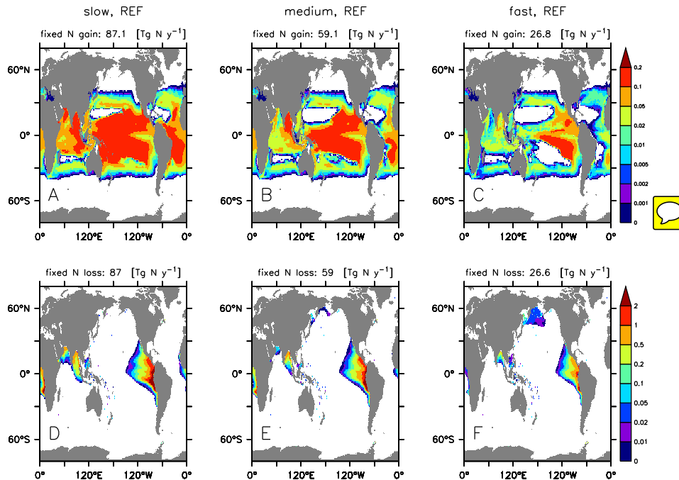
Figure 6. Vertically integrated nitrogen fixation ( \text{mmol m}^{-2} \text{d}^{-1} , panels a–c), and vertically integrated denitrification ( \text{mmol m}^{-2} \text{d}^{-1} , panels d–f), for reference setup REF with three different particle sinking speeds “slow” (panels a, d), “medium” (panels b, e) and “fast” (panels c, f). Note non-linear colour scales. Numbers on top of each panel give global integrated flux of year 9001.
