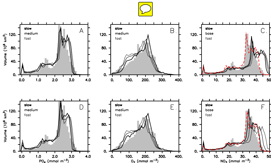
Figure 3. Volume distributions of global phosphate (panels a , d ), oxygen (panels b , e ) and nitrate (panels c , f ) for model BUR of Kriest and Oschlies (2013, upper panels a–c ), and experiment REF of MOPS (lower panels d–f ). Grey bars denote the corresponding observations (Garcia et al., 2006a, b). Lines thickness denotes different sinking speeds. Thick: slow sinking. Medium: medium sinking. Thin: fast sinking. Nitrate for model BUR (without nitrogen cycle) has been calculated from phosphate \times 14.28 . In addition, we present nitrate calculated from phosphate \times 14.28 for the “slow” sinking scenario as thick dashed red lines.
