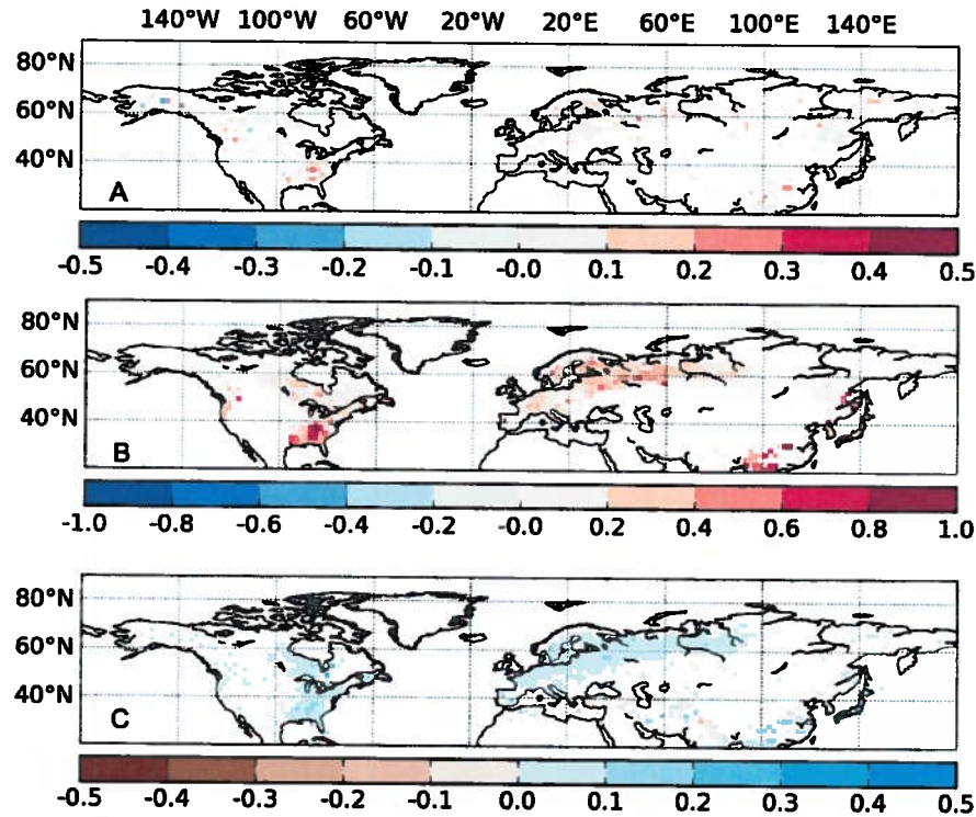
Figure 13. Difference of tree fractional cover (a), tree NPP ( \text{gCm}^{-2}\text{yr}^{-1} , b) and water availability (WA, c) between with and without \text{CO}_2 rising (NEW-EXP2). NPP is averaged over tree PFTs (PFT 2–9) weighted by their fractions. WA is averaged over the growing season (May–September) and over tree PFTs (PFT 2–9) weighted by their fractions.
