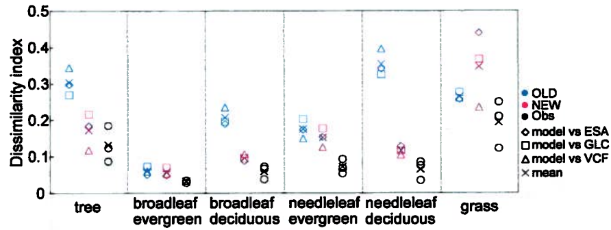
Figure 7. Dissimilarity index ( D , Eq. 10) for fractional cover of PFT groups including total tree, grass, and four tree subtypes between model (OLD, blue, and NEW, red) and observations, and between different observations (black), averaged over Northern Hemisphere ( 20\text{--}90^\circ\text{N} ). D ranges from 0 to 1, with higher values representing larger disagreement.
