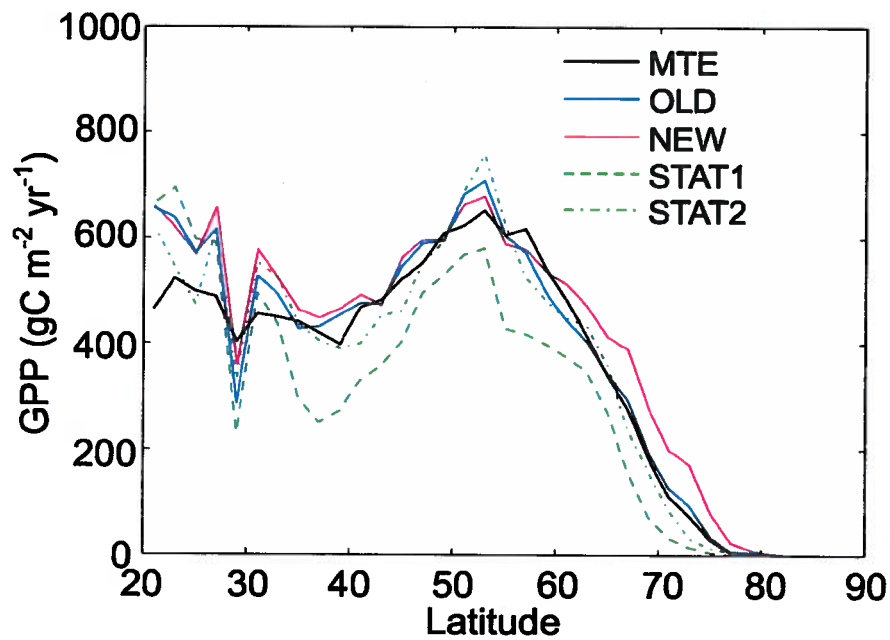
Figure 10. Latitudinal mean annual GPP (2° bands) during 1999–2008 from OLD (blue) and NEW (red), compared with that from STAT (static run in which ORC-VD is deactivated, green dashed lines) and MTE (Jung et al., 2011, black). In STAT1 and STAT2, PFT map is prescribed from ESA and SYNMAP respectively.
