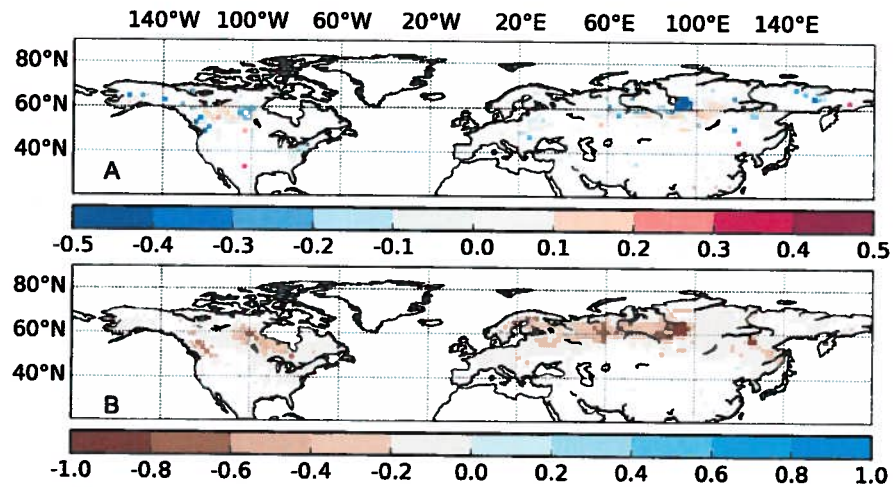
Figure 12. Difference of tree fractional cover (a) and water availability (WA, b) between with and without soil freezing (NEW-EXP1). WA is averaged over the growing season (May–September) and over tree PFTs (PFT 2–9) weighted by their fractions.
