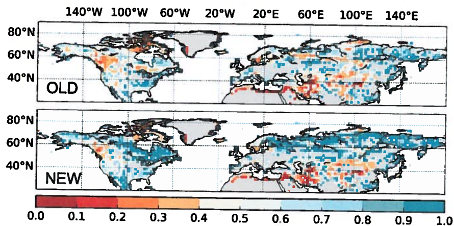
Figure 6. Model skill at simulating vegetation distribution ( S_V , Eq. 9) for OLD and NEW. S_V ranges from 0 to 1, with higher values representing better model performances, integrating observational uncertainty. Three kinds of grid cells are masked out (in gray): (1) the grid cells where S_V > 1 for both models, indicating that the observational data have too large uncertainties to be qualified for model evaluation (13% of the total land points for the studied region), (2) the grid cells where all models and datasets have 100% bare ground in Sahara Desert and Greenland (10%), and (3) the grid cells where crop fraction is higher than 0.5 (8%).
