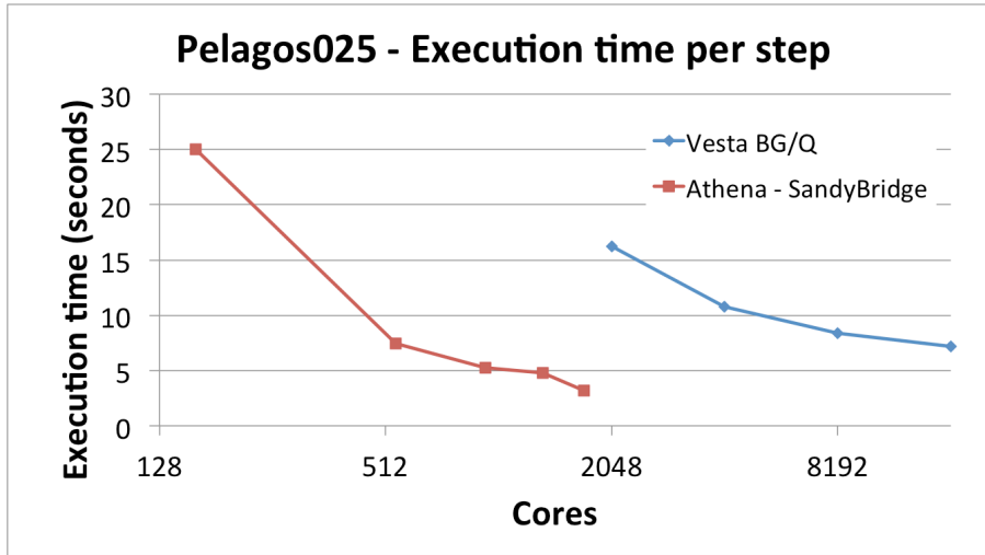
Figure 3. Scalability of PELAGOS025 configuration: comparison between the results obtained on ATHENA and VESTA. The red line represents the execution time for a time step of the model on ATHENA, the blue line on VESTA.
