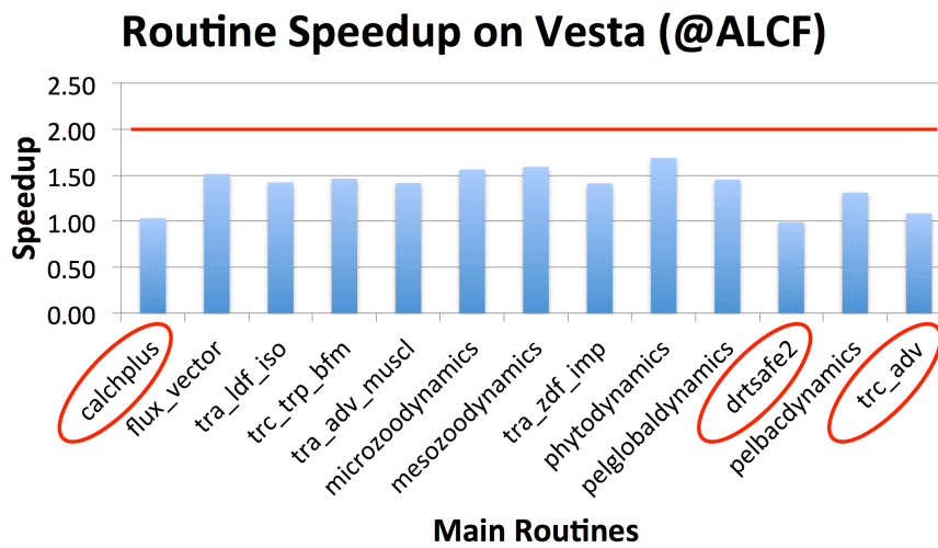
Figure 6. Analysis of scalability of the main routines on the iDataPlex-BG/Q cluster in terms of speedup. The speedup is evaluated as ratio between the execution time on 2048 and 4096 cores. Hence the ideal scalability is reached with speedup equal 2. The red circles indicate the routines whose speedup is far from the ideal value.
