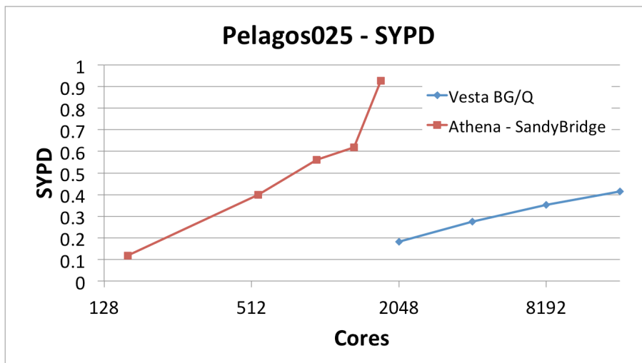
Figure 4. Scalability of PELAGOS025 configuration: comparison between the results obtained on ATHENA and VESTA. The red line represents the Simulated Years Per Day of the model on ATHENA, the blue line on VESTA.
