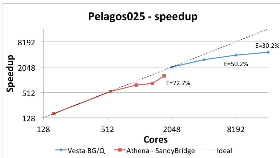
Figure 2. Scalability of PELAGOS025 configuration: comparison between the results obtained on ATHENA and VESTA. The red line represents the speedup of the model on ATHENA, the blue line on VESTA. The dashed line represents the ideal speedup.
