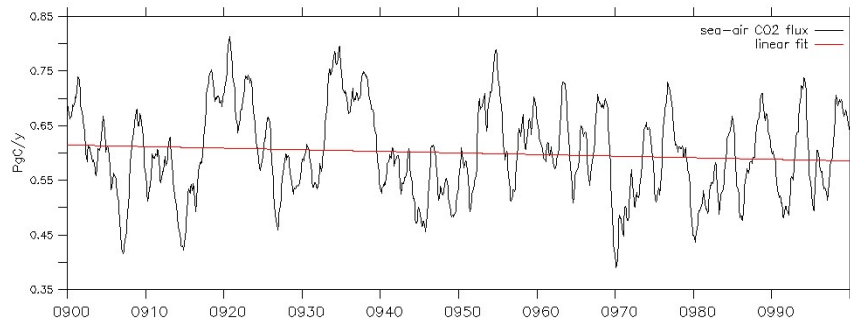
Fig. 2. Sea-air CO 2 flux from year 900-1000 (black) and linear fit (red)
