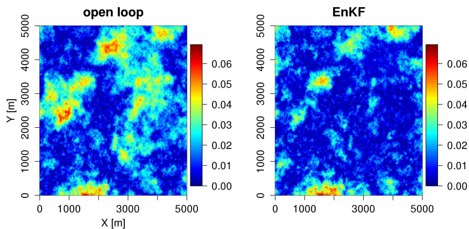
Fig. 2. Absolute average error of soil water content for open-loop (left) and assimilation (right) at a depth of -65\text{ cm} from April–June 2013.
