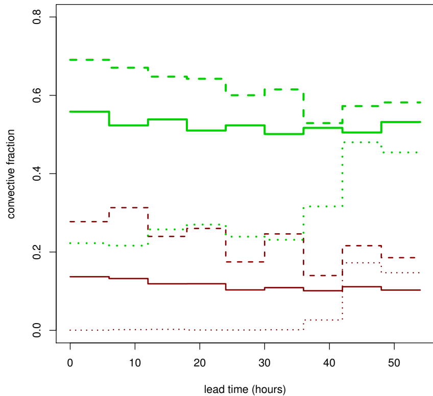
Fig. 7. Convective fraction for weakly-forced cases (dashed lines), strongly-forced cases (dotted lines) and overall (solid lines) for GR (green) and PC (red)
