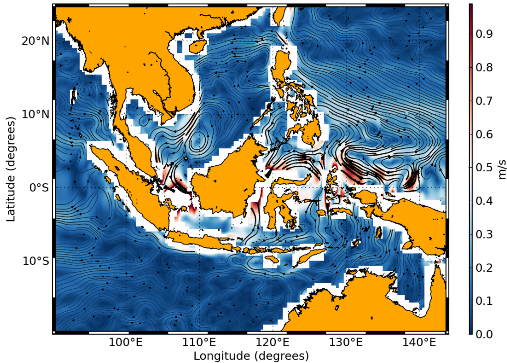
OSCAR surface currents DJF (2008_2013)
