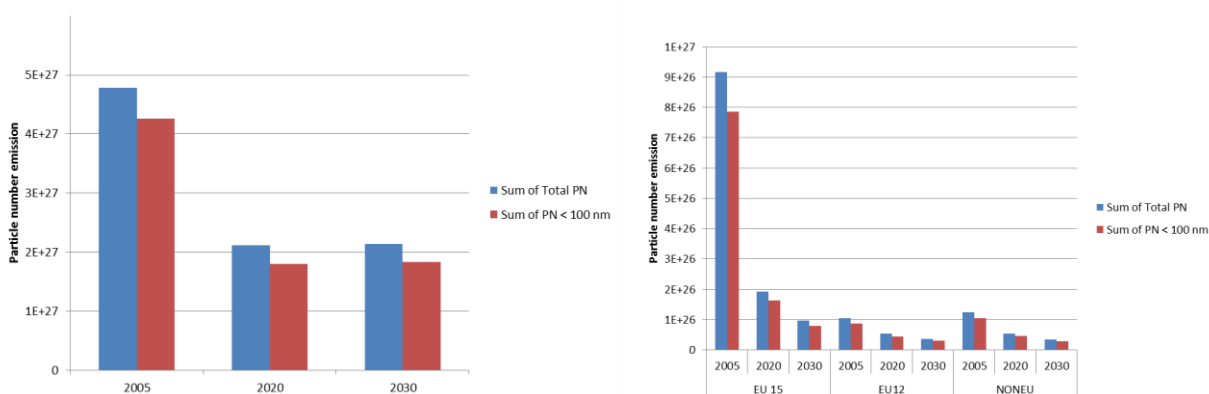
Figs. 3a-b. (a) Total anthropogenic particle number emissions and total particle number emissions in the particle size range of 10-100 nm for UNECE-Europe for 2005, 2020 and 2030 and (b) the same emissions exclusively for road transport, segmented by country group.
