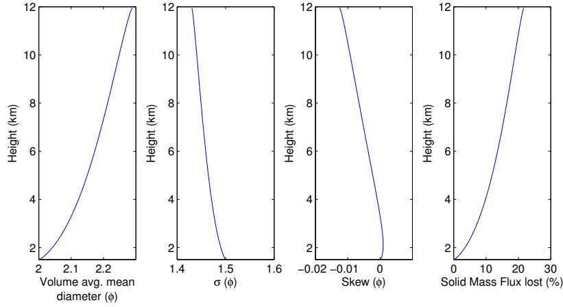
Figure 1: Particles distribution parameters (mean, variance and skewness) and cumulative loss of solid mass flux for test case 1.
