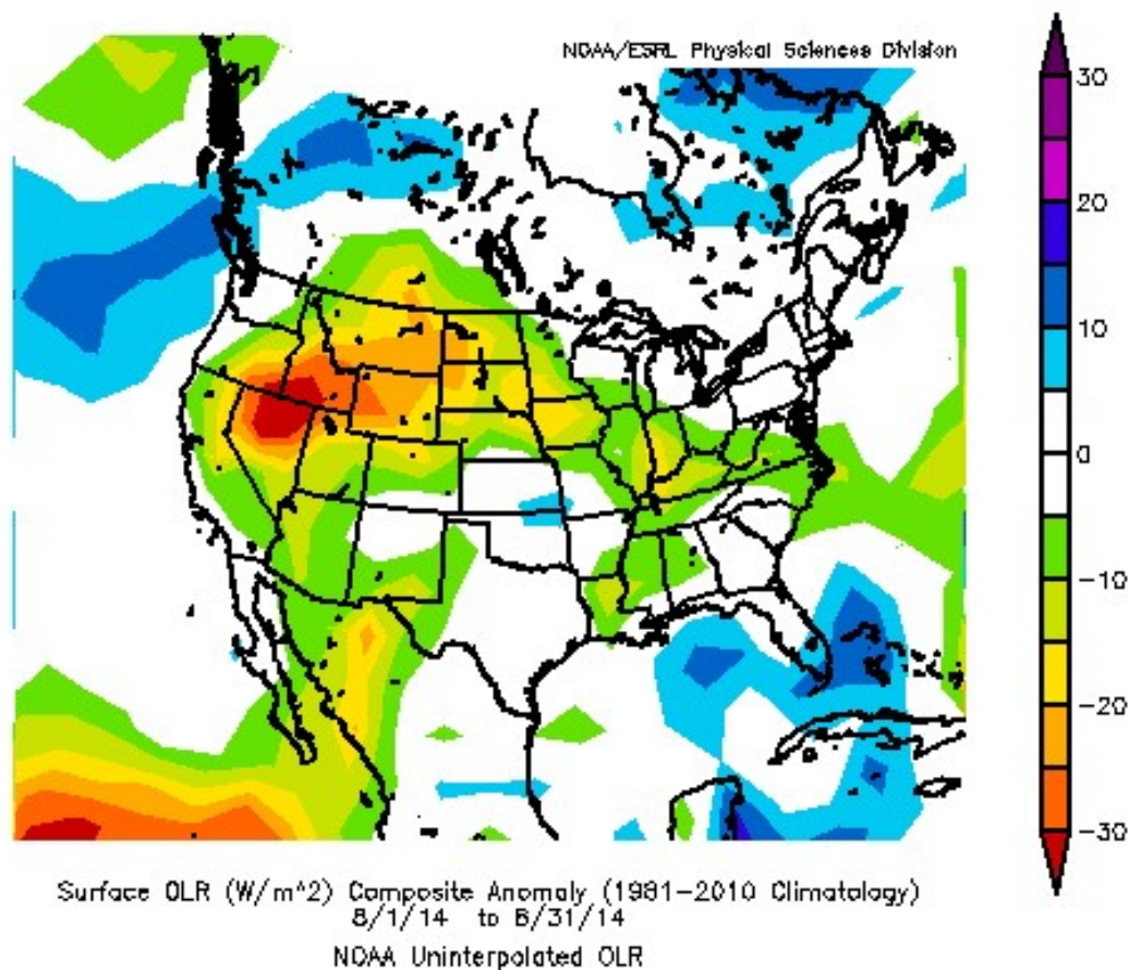
Fig. 4. august 2014, OLR anomaly
