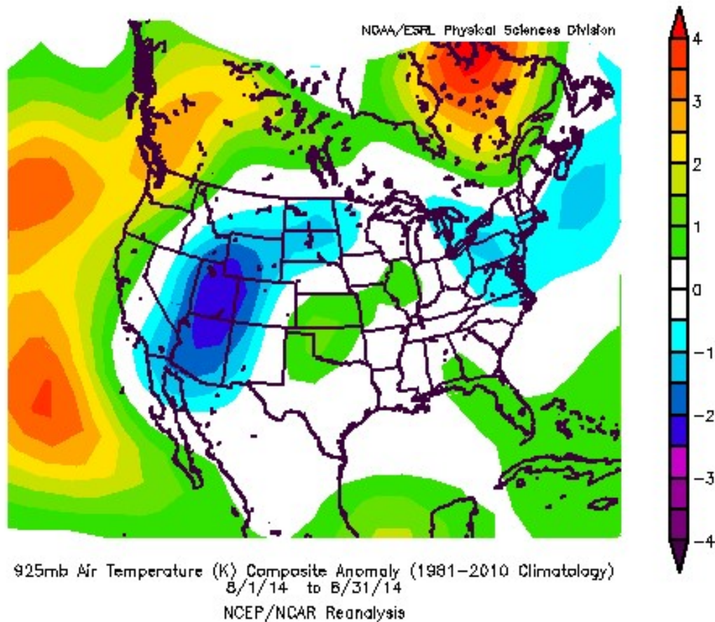
Fig. 3. august 2014, temp anomaly
