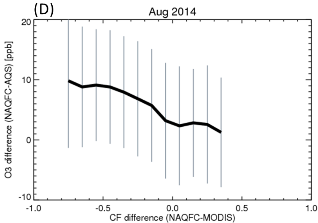
Fig. 5. Figure 3d from text
