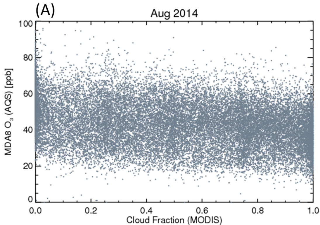
Fig. 1. Figure 3a from text
