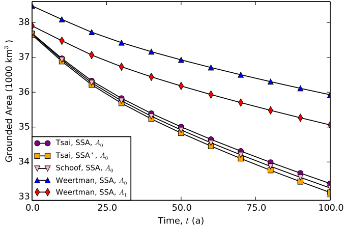
Figure 5. BISICLES Parameter sensitivity in the MISMIP+ Ice1r experiment. The Tsai et al. (2015) and Schoof (2005) basal traction laws lead to similar initial states and rates of retreat, as do the SSA and SSA* stress approximations, given the same rate factor A_0 = 2.0 \times 10^{-17} \text{ Pa}^{-3} \text{ a}^{-1} . On the other hand the, the Weertman basal traction law results in a grounding line some way upstream given the same rate factor, a closer grounding line when the rate factor is increased to A_1 = 2.2 \times 10^{-17} \text{ Pa}^{-3} \text{ a}^{-1} , and a far slower rate of retreat in either case.
