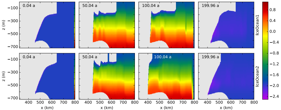
Figure 13. Example results from POPSICLES plotted as in Fig. 8 but for IceOcean1 (top) and IceOcean2 (bottom) simulations each lasting 200 years. Both simulations begin with ice shelves that are in steady state without melting and with COLD ocean conditions. The WARM far-field restoring in the ocean causes the melt rate to increase by several orders of magnitude over the first decade and for the ice shelf to thin over the remainder of the retreat phase (100 years). In IceOcean2, dynamic calving significantly reduces the size of the ice shelf compared with IceOcean1. During the final 100 years, the switch to COLD far-field restoring leads to cold ocean temperatures, melt rates are reduced by several orders of magnitude, and the ice shelf begins to re-advance. One hundred years is not long enough for the ice shelf in either simulation to re-advance to its initial steady state.
