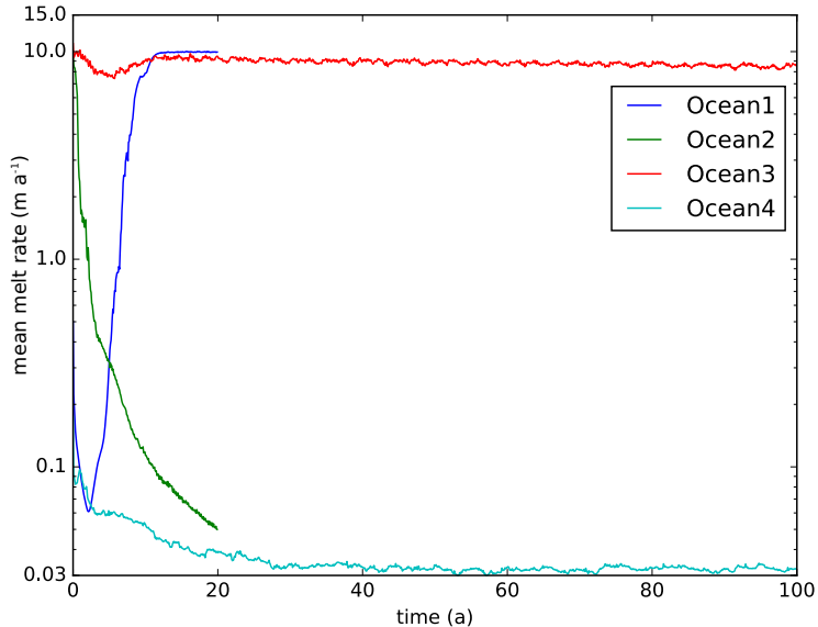
Figure 7. Example results from POP2x simulations showing melt rates averaged over the shelf area as functions of time for Ocean1–4. Melting increases by nearly two orders of magnitude in Ocean1, and decreases by about the same order in Ocean2, demonstrating that changes in far-field forcing can greatly increase or reduce melting. After a decade or two of initial adjustment, the melt rates in Ocean3 and Ocean4 remain relatively steady in time despite the changing topography in those experiments, suggesting that the total cavity size has relatively little impact on total melting.
