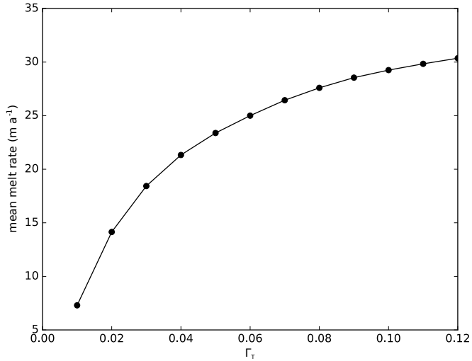
Figure 9. Example results from a series of POP2x simulations of Ocean0 showing the dependence of the mean melt rate \langle m_w \rangle averaged over locations below z_d = -300 m and over the final six months of the simulation for various values of the turbulent heat-transfer coefficient \Gamma_T . Based on these results, the value \Gamma_T \approx 0.11 , corresponding to a mean melt rate m_w \approx 30 \text{ m a}^{-1} , was used for subsequent ISOMIP+ and MISOMIP1 simulations.
