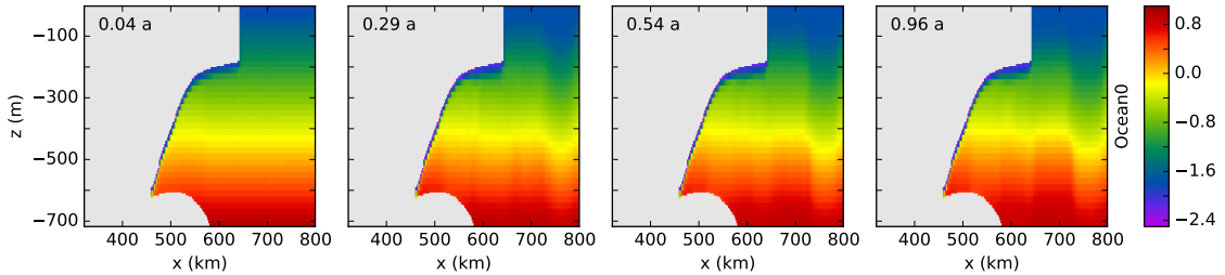
Figure 8. Example results from a 1-year Ocean0 simulation with the POP2x model using heat-transfer coefficient \Gamma_T = 0.11 . Panels show the progression in time of transects of monthly-averaged ocean temperature through the center of the domain ( y = 40 km). The initial conditions and far-field restoring at the right-hand side of the domain both use the WARM profiles from Fig. 6. The ice draft does not evolve in time. The simulation reaches a quasi-steady state with relatively strong melting within a few months.
