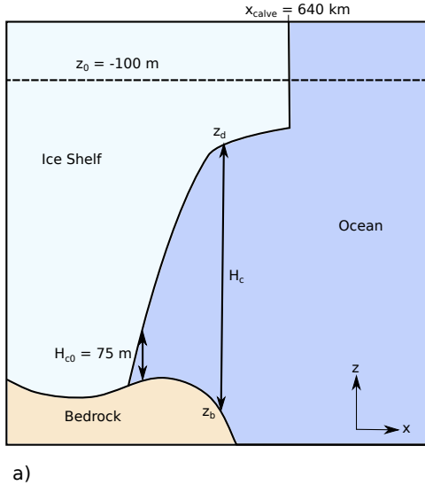
Figure 3. (a) A schematic showing the ice draft ( z_d ), the bedrock elevation ( z_b ), the cutoff depth ( z_0 ) above which the melt rate is zero, the ocean column thickness ( H_c ) and the reference thickness H_{c0} . (b) The melt parameterization given by Eq. (17). Melting increases linearly with decreasing z_d below z_0 and is independent of H_c when the ocean column is thick zero near the grounding line as the ocean column thins.
