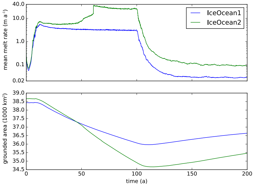
Figure 12. Example results from POPSIKLES simulations of IceOcean1 (no dynamic calving) and IceOcean2 (thickness-based calving criterion) using SSA and the sliding law from Weertman (1974) showing melt rates averaged over the shelf area (top panel) and the grounded area as functions of time (bottom panel). Though melt rates are initially similar, after about year 40 the dynamic calving in IceOcean2 begins to remove substantial areas of the ice shelf (notably when an iceberg is removed just after year 60), resulting in larger mean melt rates (but similar total melt fluxes) for that experiment. IceOcean2 loses substantially more grounded area than IceOcean1 during retreat (the first 100 years), presumably due to a loss of buttressing from the ice shelf, which has nearly completely calved away. The grounding line re-advances at approximately the same rate in both experiments because the advancing shelf is thick enough not to calve.
