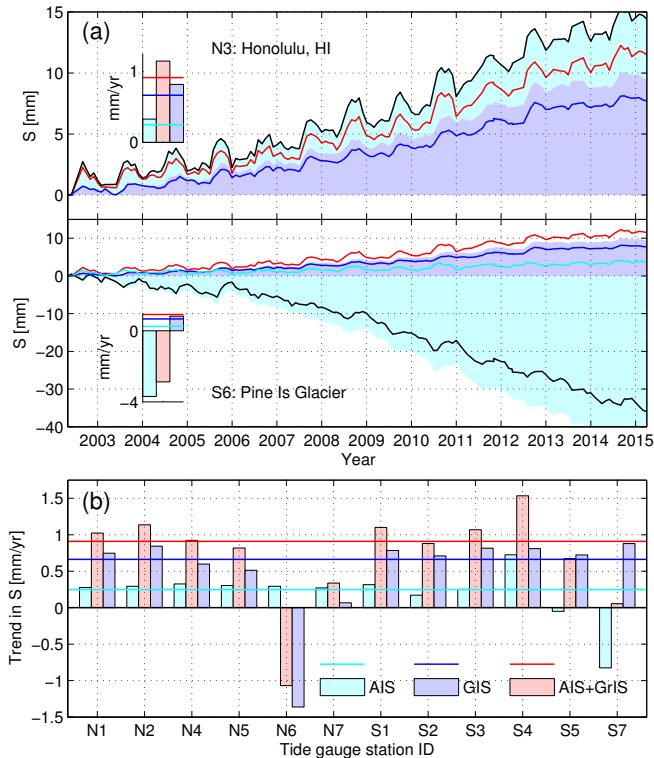
Figure 5. Magnitudes and trends of sea level change at 14 selected locations. (See Table 3 for their description and Fig. 4a for locating their position on the global map.) (a) Change in relative sea level over time at two representative sites. Average rates of relative sea level change are also shown in the insets. (b) Rate of change in relative sea level, averaged over the GRACE period, at 12 other locations. Cyan and blue colors (both fill and line) represent the contribution from the AIS and GrIS, respectively. The combined contributions of ice sheets are shown in red. Black lines in Fig. 5a represent the local values and all others denote the global mean values.
