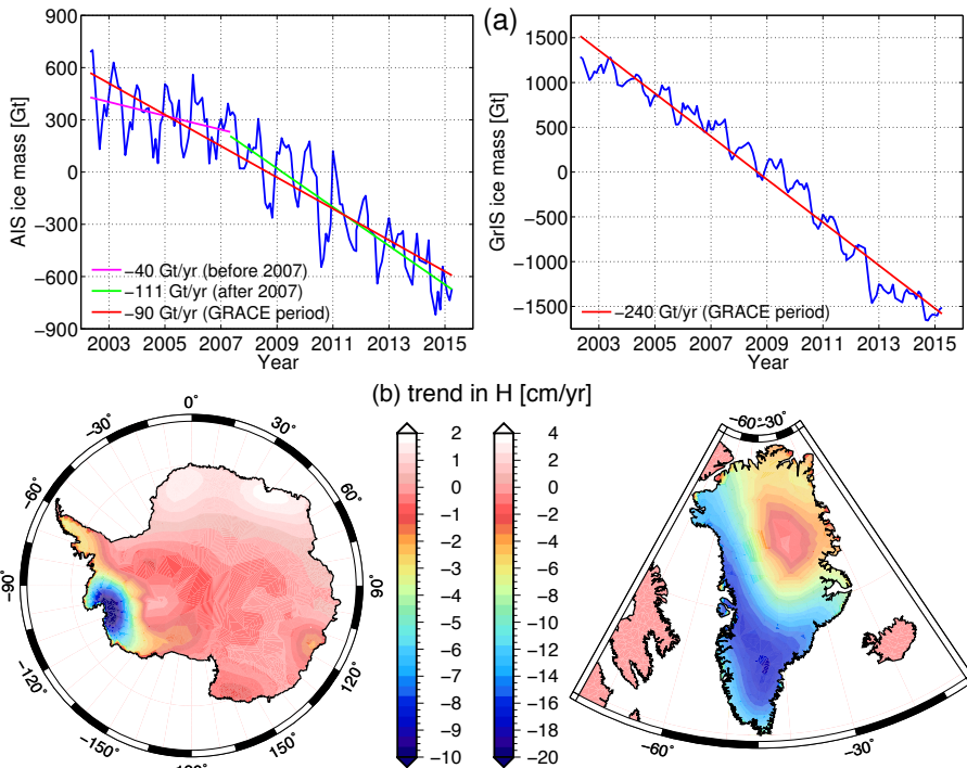
Figure 3. Summary of the GRACE data used in this study. (a) Ice mass change in the AIS and GrIS from April 2002 to March 2015. (b) Spatial distribution of rate of change in ice thickness, averaged over the GRACE period. See Sect. 4.1 for a detailed discussion of the GRACE data processing.
