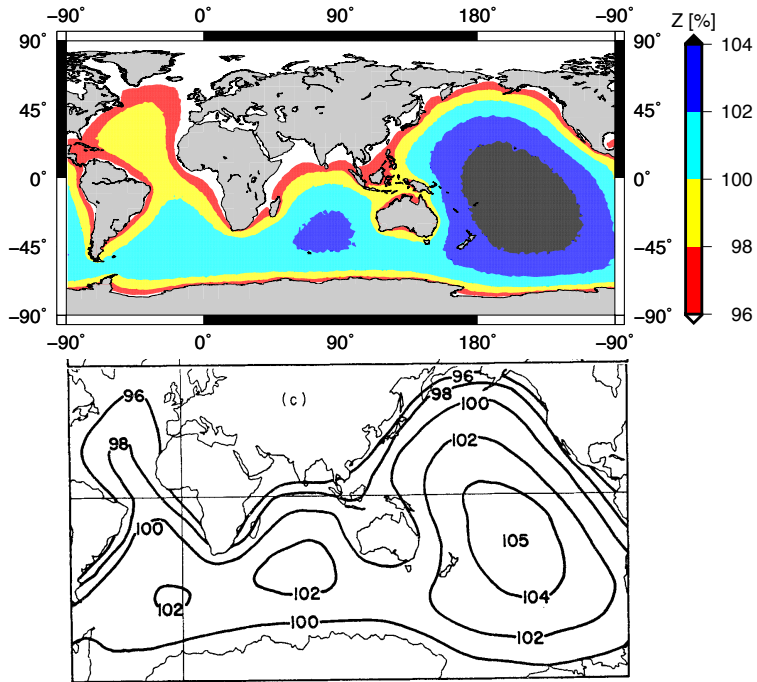
Figure B1. Change in relative sea level neglecting ice loads on an elastic non-rotating earth. Normalized sea level with respect to global mean value (see Eq. B1), (a) computed by ISSM-SESAW and (b) provided by Farrell and Clark (1976).
