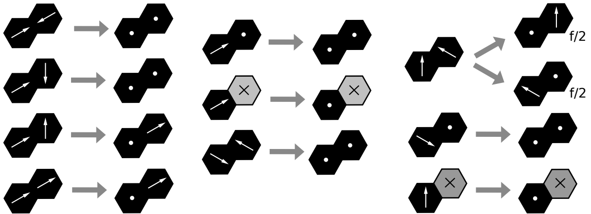
Figure 13. Friction rules for lattice-grain model. Unless otherwise noted, each transition has a rate f , whereas the corresponding transition rates for elastic behavior (Figure 11) have rate e = 1 - f .
