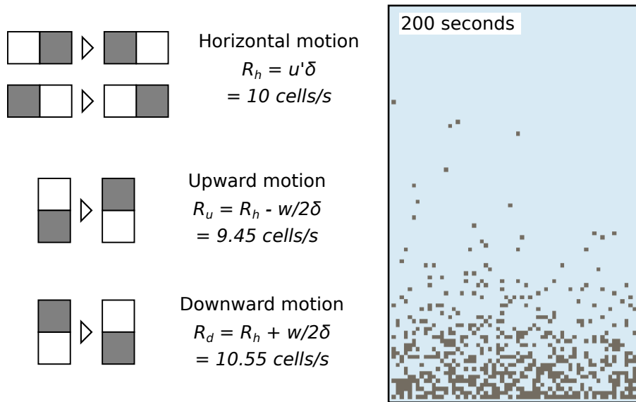
Figure 2. Turbulent suspension model with grains (1 mm tea leaves) that are 0.2% denser than the surrounding fluid. Left: illustration of cell-pair transitions representing motion in the four directions. Grain settling velocity of 0.0011 m/s imparts asymmetry to the transition probabilities.
