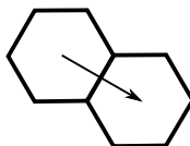
Figure 5. Illustration of cell-pair orientations and corresponding orientation codes. Arrows represent links, each of which connects a tail node to a head node .
