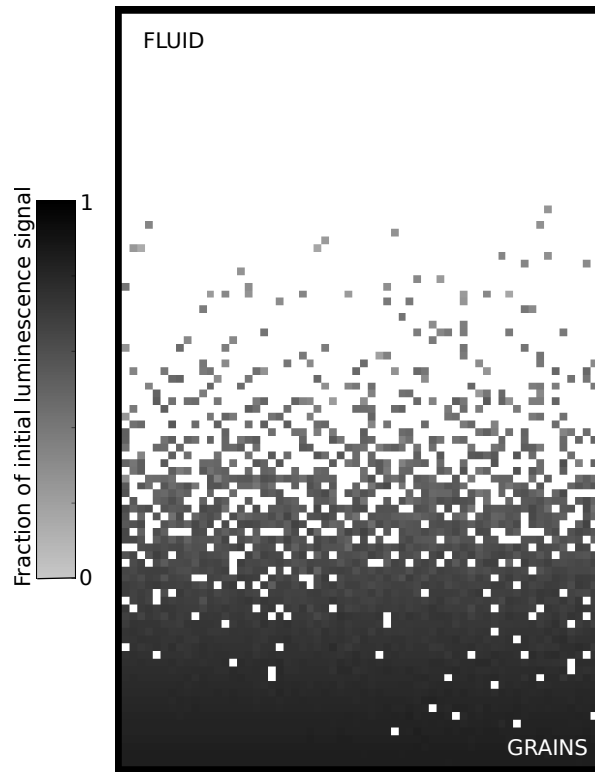
Figure 8. Model of turbulent sediment suspension, showing the computed luminescence signal after 20 seconds of stirring and bleaching. The original luminescence signal is removed (bleached) by exposure to light. Because light intensity declines exponentially from top to bottom, grains near the bottom are less fully bleached than those near the top. Turbulent mixing disperses the partially bleached grains.
