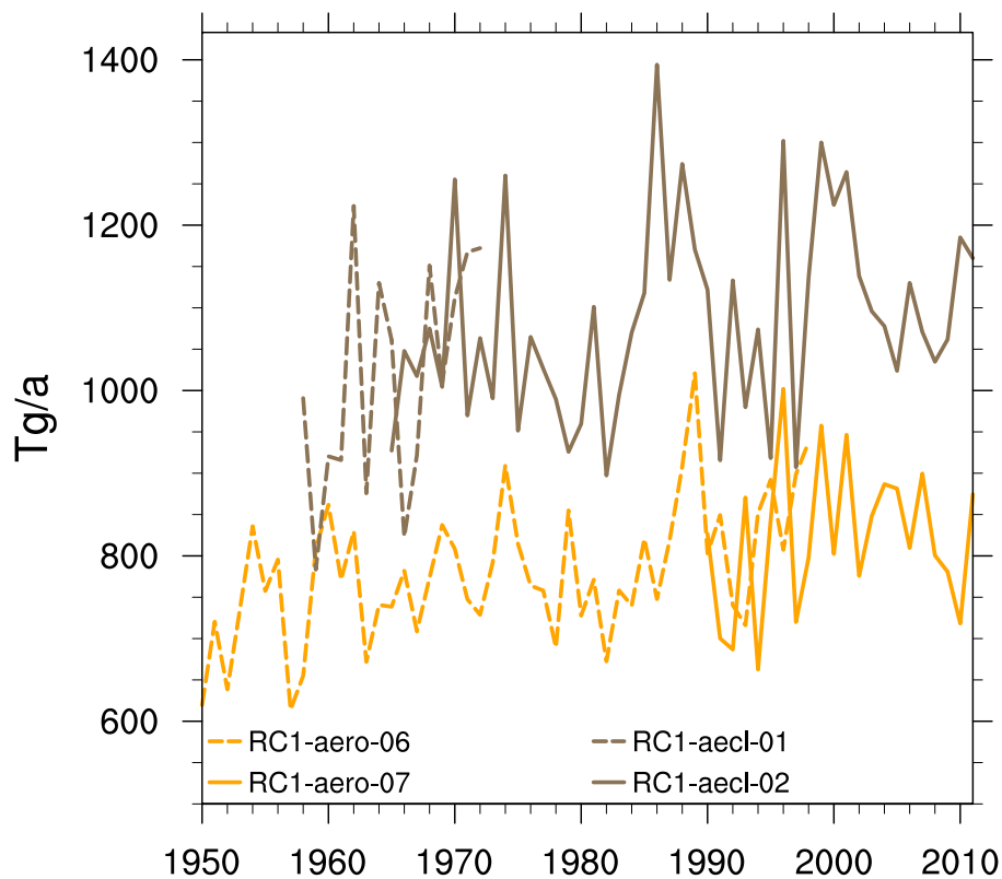
Figure 10. Annual total emissions of dust (in \text{Tg a}^{-1} ) as calculated in the RC1-aero and RC1-aecl simulations.
