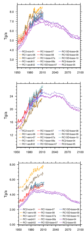
Figure 16. Globally integrated annual nitrate dry deposition (upper), wet deposition (middle) and sedimentation (lower) fluxes in \text{Tg(N)}\text{a}^{-1} .
