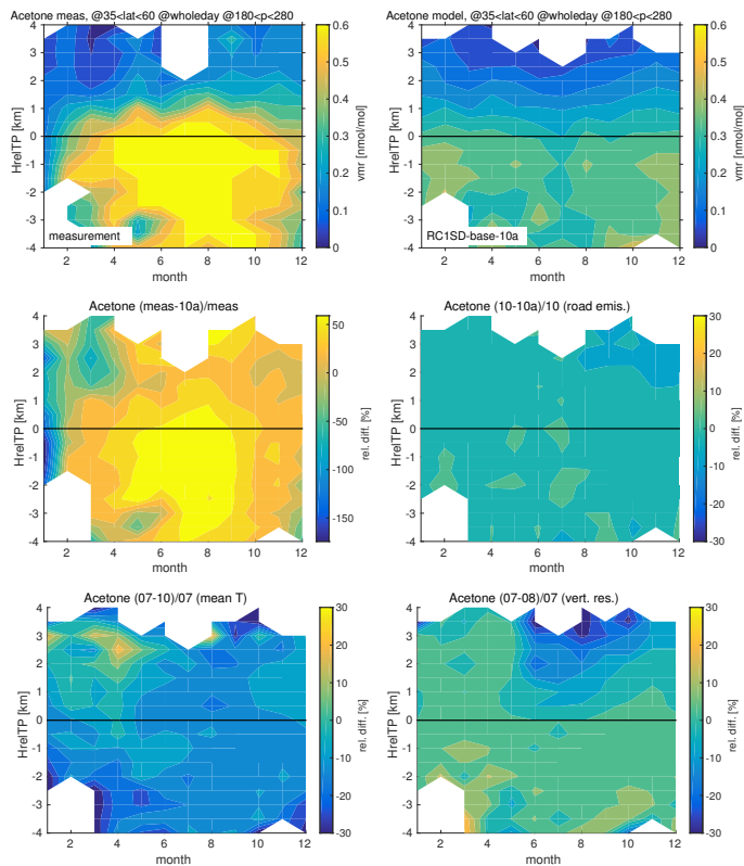
Figure 22. As Fig. 19, but for acetone.
