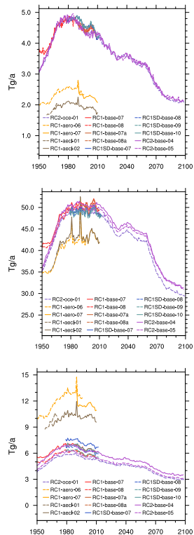
Figure 17. Globally integrated annual non-sea salt sulphate dry deposition (upper), wet deposition (middle) and sedimentation (lower) fluxes in \text{Tg(S)}\text{a}^{-1} .
