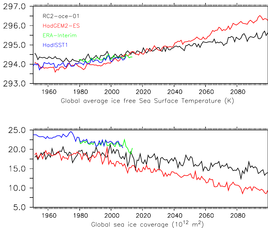
Figure 11. Global annual average (ice free) SSTs (in K, upper panel) and SIC (in 10^{12} \text{ m}^2 , lower panel) of simulation RC2-oce-01 (1950–2099, black) compared to prescribed SSTs/SICs of simulations RC1-base (HadISST, blue), RC2-base (HadGEM2-ES, red) as described in Sect. 3.3, and of ERA-Interim (green) as applied in the nudged simulations RC1SD-base .
