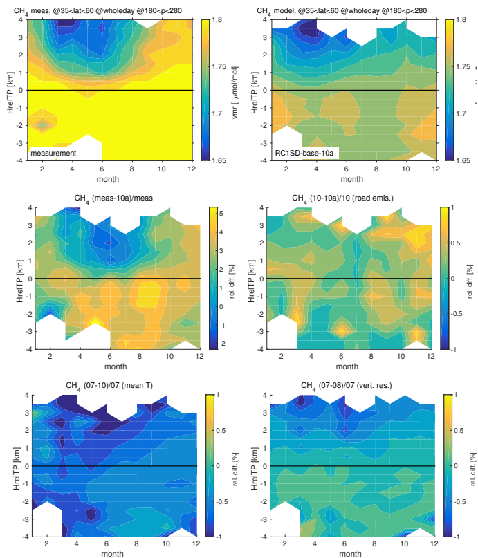
Figure 21. As Fig. 19, but for CH 4 .
