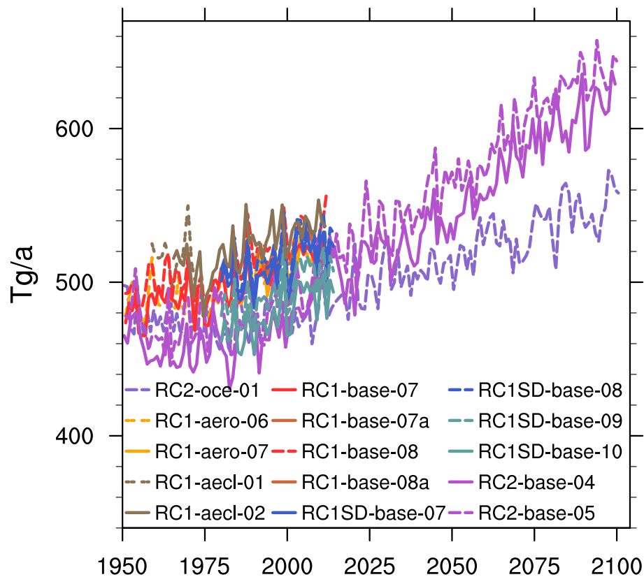
Figure 3. Annual total emissions of on-line calculated biogenic isoprene emissions in \text{Tg(C)a}^{-1} .
