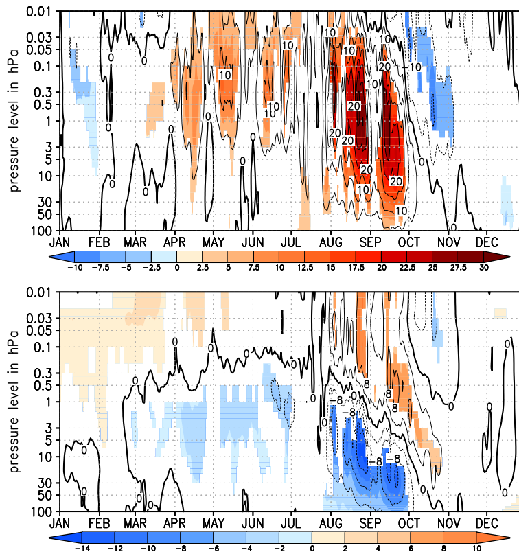
Figure 1. Differences of the daily mean climatology (19 years) between a T42L47MA EMAC simulation with the gravity wave parameter rm_\text{scon} set to 0.92 in comparison with a simulation where it is set to 0.96; for the zonal mean zonal winds at 60^\circ\text{S} in \text{m s}^{-1} (top); for the zonal mean temperatures averaged from 71.2\text{--}87.9^\circ\text{S} in K (bottom). The shading indicates the differences that are significant at the 95 % level, estimated with a Student's t test.
