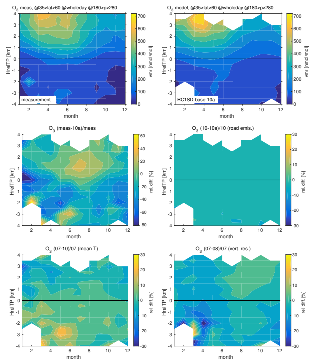
Figure 19. Comparison of O_3 climatologies based on data from the years 2005–2013. The first row shows climatologies of CARIBIC measurements (left) and RC1SD-base-10a model data (right). The second row shows the relative differences of measurements and model data (left) and the relative differences between RC1SD-base-10a and RC1SD-base-10 , which differ in road traffic emissions (right). The bottom row shows the relative differences of RC1SD-base-07 and RC1SD-base-10 , differing in nudging of global mean temperatures (left), and the relative differences of RC1SD-base-07 and RC1SD-base-08 , with different vertical resolutions (right). The vertical axis shows the distance (in km) relative to the tropopause.
