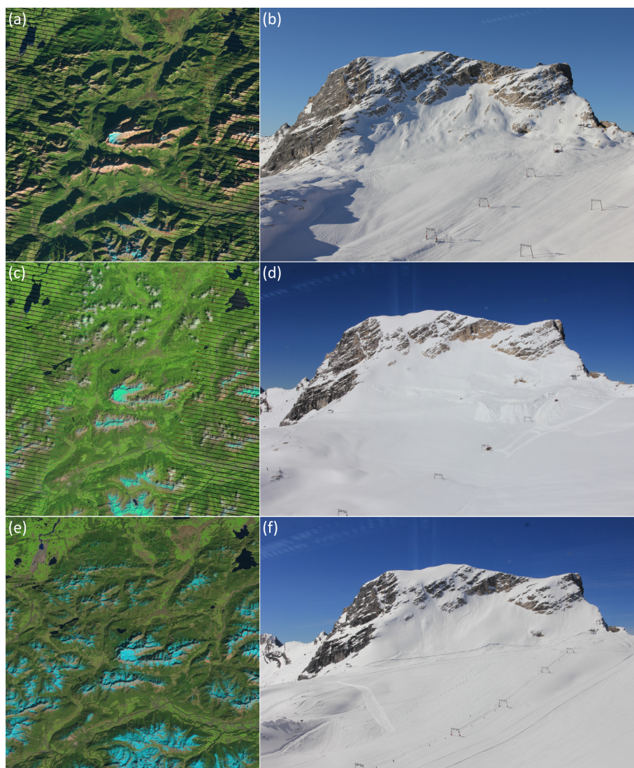
Figure 2. Enlarged view of the landsat look images of Zugspitzplatt (in the centre) and SLR photographs of Schneefernerkopf for 17 November 2011 ( a and b ), 1 July 13 2013 ( c and d ) and 7 April 2014 ( e and f ): snow cover extents are generally depicted in cyan colors in the Landsat scenes. ( a ) and ( b ) show about one month old snow with strong shadowing effects and some partial cloud coverage (not visible in the Landsat Look image). ( c ) and ( d ) display fresh snow and have a significant but partial cloud coverage. ( e ) and ( f ) also show fresh snow but under clear conditions and with some weak shadowing effects.
