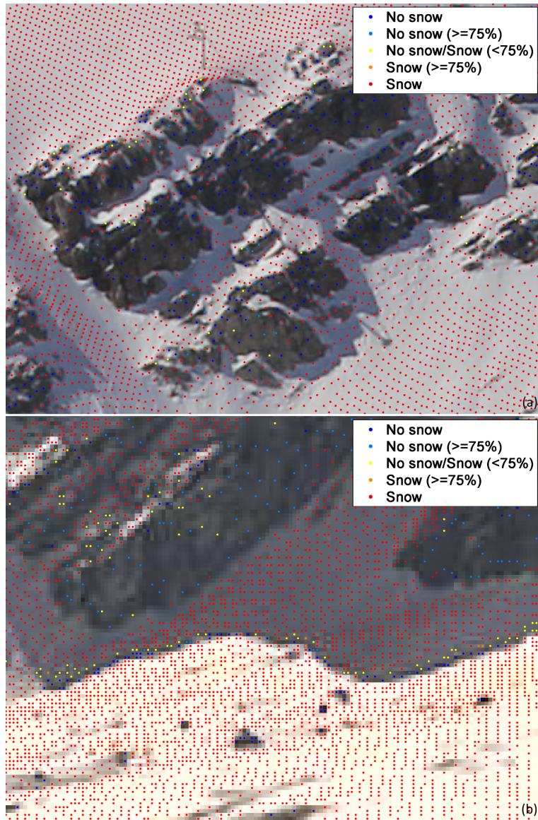
Figure 11. Enlarged view of the superimposed snow classifications on the SLR and webcam photographs of 7 April 2014 (rectangle boxes in Fig. 11c and d): (a) unsure classification results in the SLR photograph are located at transitional areas between snow patches and snow-free areas. (b) In the webcam photograph, more pixels are classified in the three “unsure” categories. Moreover, some “no snow” misclassifications are found at the transitional zone between sunny and shaded snow cover.
