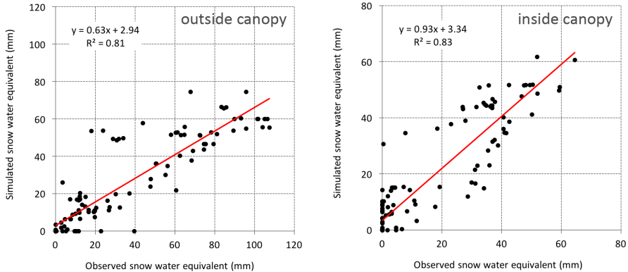
Figure 13. Snow water equivalent simulated with ESCIMO.spread (v2) vs observed snow conditions out- and inside the forest canopy for the winter period 2012/13 at site Vordersteinwald.
