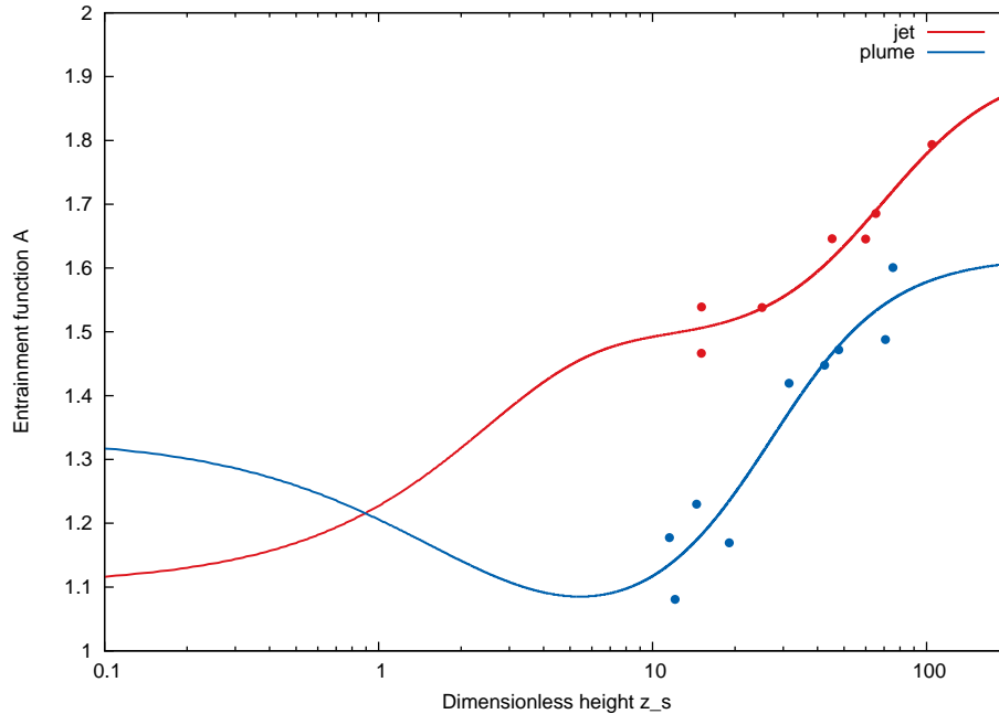
Figure 2. Entrainment functions A(z_s) for jets and plumes depending on the dimensionless height z_s = z/2r_0 . Functions have been obtained by fitting experimental data (points) from Carazzo et al. (2006) (for z_s > 10 ) and multiplying by a correction function (20c) to extend the functions to z_s < 10 verifying function continuity and convergence to values of A = 1.11 for jets and A = 1.31 for plumes when z_s \rightarrow 0 .
