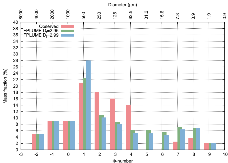
Figure 11. Grain size distribution predicted by the wet aggregation model for Eyjafjallajökull 6 May phase for a column height of 7 km (a.v.l.) for two different values of the fractal exponent D_f of 2.95 and 2.99. Observed data from Bonadonna et al. (2011).
