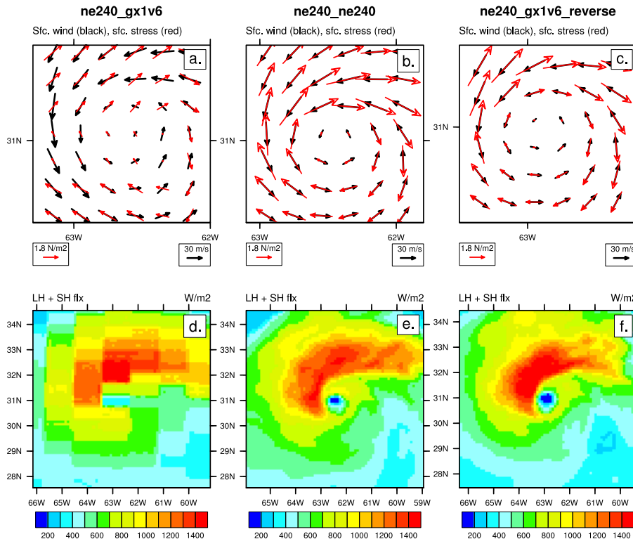
Figure 5. 120-hour CAM-SE forecast for Hurricane Leslie, valid at 00Z on 5 September 2012. Left panels (a, d) are results from forecast using 1° ocean grid in the default configuration (calculations carried out on ocean grid). Center panels (b, e) show results using 0.125° ocean grid. Right panels show version of 1° grid where calculations are carried out on the atmospheric grid. Top panels (a–c) display instantaneous wind in the lowest model (black vectors) with corresponding lowest model level wind stress (red vectors). Lower panels (d–f) show total surface flux (latent plus sensible heat).
