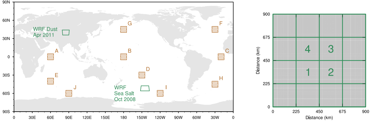
Figure 1. Left panel indicates the two 900 \text{ km} \times 900 \text{ km} WRF domains (green), and the ten 10^\circ \text{ lat} \times 10^\circ \text{ lon} regions (brown) in which the estimated sub-grid wind variabilities are evaluated in Fig. 8. Right panel shows the four imagined 225 \text{ km} grid boxes (label as 1–4) in each of the WRF domains shown in the left panel. The 225 \text{ km} grid boxes are used for the offline estimates in Figs. 4 and 6, as well as the evaluations in Figs. 9 and 11.
