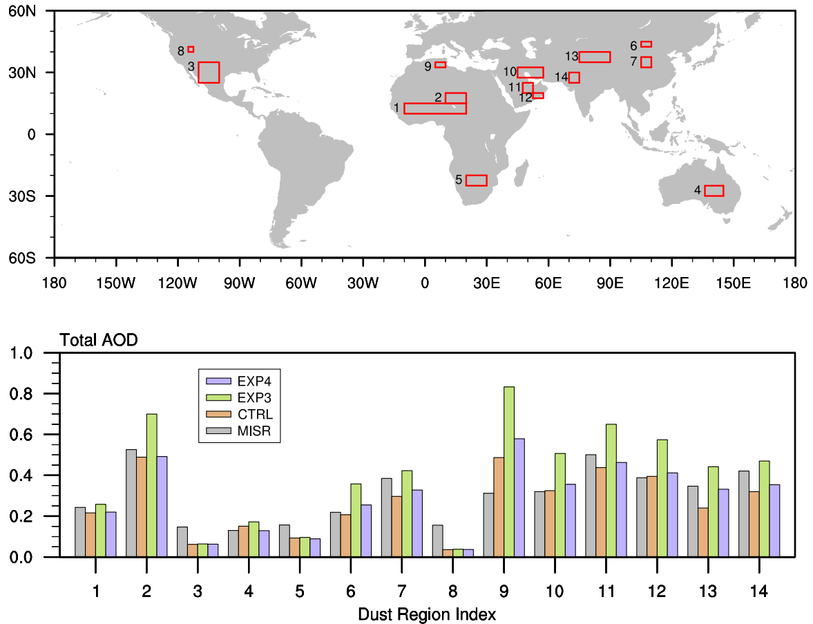
Figure 17. Satellite retrieved AOD from MISR (Multi-angle Imaging Spectro-Radiometer) and simulated regional average AOD at 550nm at 14 major dust source regions ( \text{Tg yr}^{-1} ) for the year 2006. These regions were defined in the work of Zender and Kwon (2005) based on the dust source regions identified by Prospero et al. (2002) and data from Torres et al. (2002). Region definition and the data used to plot the lower panel are given Table 4.
