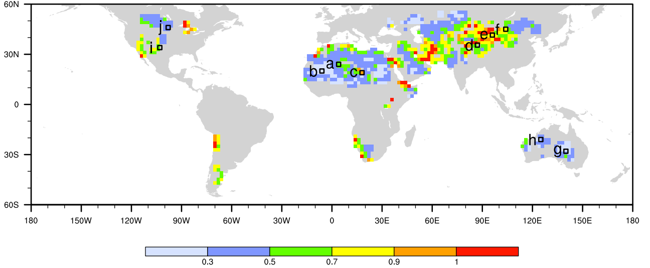
Figure 10. Geographical distribution of the coefficient D (unitless) derived for a 2^\circ lat \times 2^\circ lon GCM grid using the ECMWF 15 km analysis of the year 2011 and Eq. (26). The locations with no results are either covered by land ice or lake, or associated with leaf area indices (LAI) larger than 0.3 throughout the year, thus cannot have dust emission according to the parameterization of Zender et al. (2003) and the land surface characteristics data used in the CAM5 simulations in this paper. The black boxes correspond to the panels in Fig. 11 in which time series of sub-grid wind variability are analyzed.
