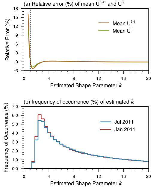
Figure 7. (a) Relative error in \overline{U_{10}^{3.41}} and \overline{U_{10}^3} as a result of estimating the shape and scale parameters of a Weibull distribution using Eqs. (15) and (16). (b) Histograms of the Weibull shape parameter k estimated with Eq. (15) using 6 hourly ECMWF analysis of January and July 2011 for imagined 2^\circ grid boxes. Further details can be found in Sect. 4.1.
