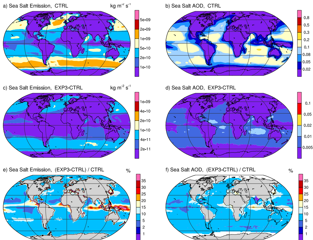
Figure 15. Top row: year 2006 mean sea salt emission flux ( \text{kg m}^{-2} \text{s}^{-1} ) and sea salt AOD (unitless) at 550 nm in the nudged CAM5 simulation (CTRL); Second row: differences between EXP3 and CTRL. Bottom row: relative differences between EXP3 and CTRL. In the bottom row, locations that have emission fluxes less than 1 \times 10^{-12} \text{ kg m}^{-2} \text{ s}^{-1} or sea salt AOD < 0.01 in the CTRL simulation are masked out.
