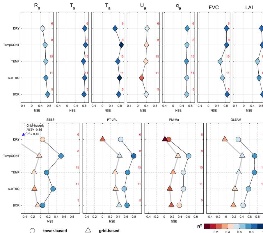
Figure 10. The upper panel shows Nash-Sutcliffe Efficiency (NSE; x axis) and R^2 (color tone) between tower-based and grid-based values for net radiation, land surface temperature, air temperature, wind speed, specific humidity, fractional vegetation cover and leaf area index across the five different climate zones. The lower panel shows NSE ( x axis) and R^2 of model simulated evaporation against closure-corrected observed values across climate zones. The number of towers for each biome are shown in red font on the secondary (right) axis of the plots. Statistics for the grid-based SEBS result over dry climate zone are printed.
