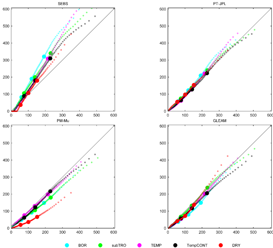
Figure 9. Percentile plots of observed ( x axis) versus estimated latent heat flux ( y axis) at 3-hourly resolution for tower-based analysis and across the different climate zones. Percentiles encompass the 1st to 99th range in 1 percent increments. Q_{25} , Q_{50} and Q_{75} are denoted by large circles.
