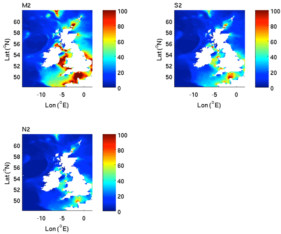
7 Figure S1. Amplitudes ( \text{cm s}^{-1} ) of the M2, S2 and N2 constituents of the local tidal 8 current vector on and around the northwest European shelf (as also used for the 9 configurations around Scotland and in the Western English Channel).
