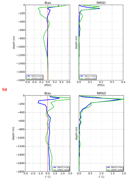
Figure 21e. Bias and RMSD of salinity (up) and temperature (bottom) between INDOMIX data and INDO12 (blue line) and parent model PSY3 (green line) at S4 location. Data are binned in 25m depth intervals for the first 100 meter depth and in 50 m depth interval for deeper layers.
