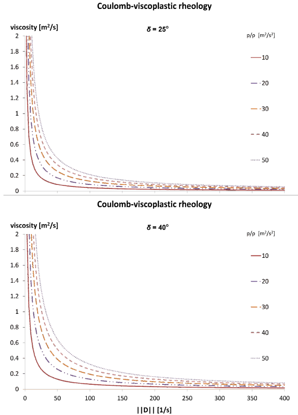
Figure 4. Dependency of the kinematic gravel phase viscosity (for friction angle \delta = 25^\circ and 50° 40° ) on the norm of the strain rate tensor ||D|| at different levels of pressure normalized by density, for m_y = 0.2 m_u = 1 s.
