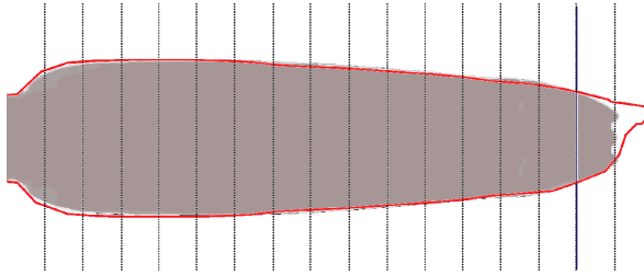
Figure 7. Simulated deposit (view from top in a hillslope debrisflow flume experiment) for a mixture with 28.5% water content and \delta = 36^\circ . The thick solid lines indicate the experimental deposit and vertical thin lines represent the 20 cm spacing marks in the experimental slope.
