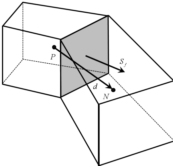
Figure 9. Sketch of two adjacent cells P and N and the shared face f owned by cell P . S_f is the face surface normal vector while d denotes the distance vector from cell center P to cell center N .
