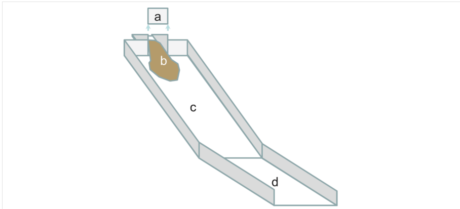
Figure 5. Iso-view sketch of the hillslope debris-flow flume. Material (b) is released from the reservoir at the top by a sudden vertical removal of a gate (a) and flows down a steep slope (c) followed by a gently inclined run-out plane (d).
