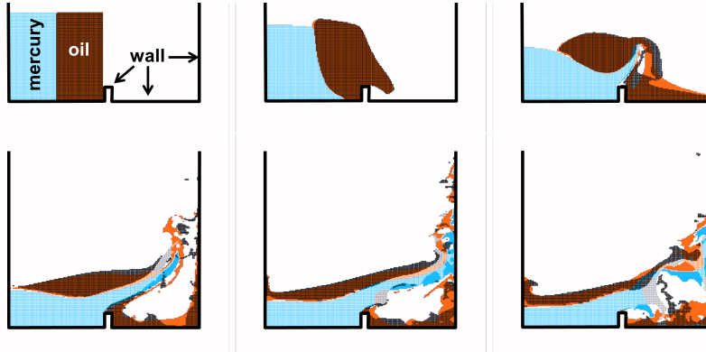
Figure 8. Phase positions in a dam break standard test-case simulation using a drag-based three phase multiphaseEulerFoam simulation (air is transparent) as background shapes with the corresponding phase positions of our model as wire frame in front (with white mercury and black oil). The visualized time steps correspond to 0, 0.1, 0.2, 0.3, 0.4 and 0.5 seconds.
