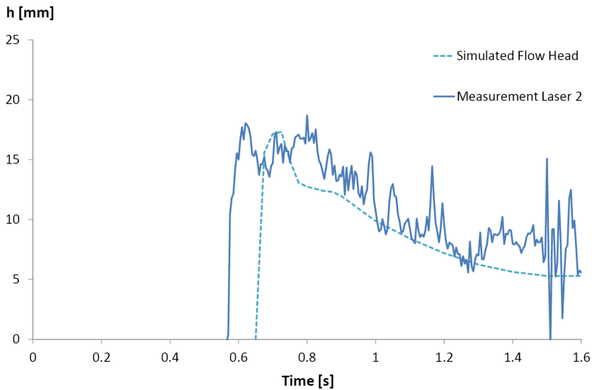
Figure 6. Laser measurement and corresponding simulated values of the flow head over time, one meter down-slope of the gate for hillslope debris-flow flume experiments with water content of 28.5%. The laser data were box-averaged over 10 milliseconds.
