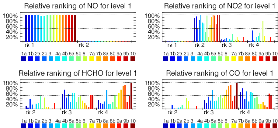
Figure 7. Relative ranking of the impact of emission uncertainties of NO (top left), NO 2 (top right), HCHO (bottom left), and CO (bottom right) for model level 1 (surface) for all 17 case studies. Plotting conventions as in Fig. 5.
