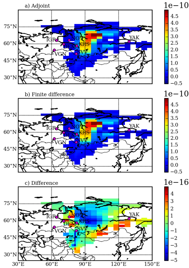
Fig. 6. Comparison of sensitivities of \text{CO}_2 concentrations ( \text{ppm}/(\mu\text{mol}/\text{m}^2\text{s}) ) for test 1: (a) sensitivity calculated considering only the Eulerian adjoint model at a resolution of 2.5^\circ , (b) the same sensitivity calculated directly from NIES forward runs using the one-sided numerical finite difference method with perturbations of \varepsilon , and c) the relative difference between derived adjoint and the numerical finite difference gradients. Magenta dots with labels depicts the locations and names of the Siberian observation towers.
