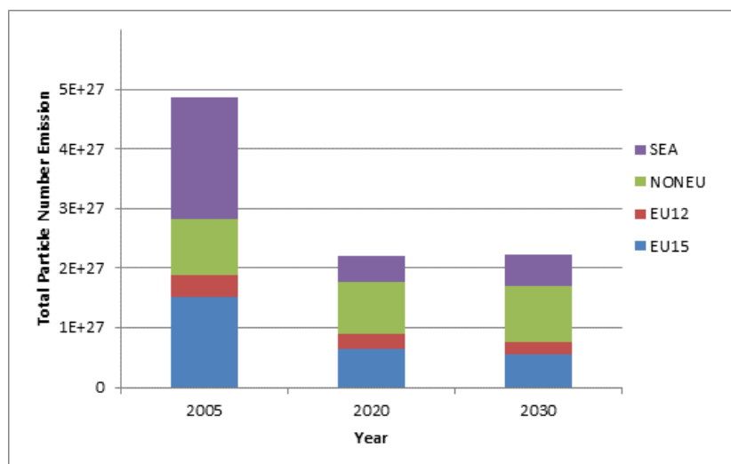
Figs. 2a-b. Total anthropogenic particle number emissions in the United Nations Economic Commission for Europe, (a) classified by the source sector for 2005, and (b) classified by the country group for 2005, 2020 and 2030. ‘Sea’ refers to international shipping.
