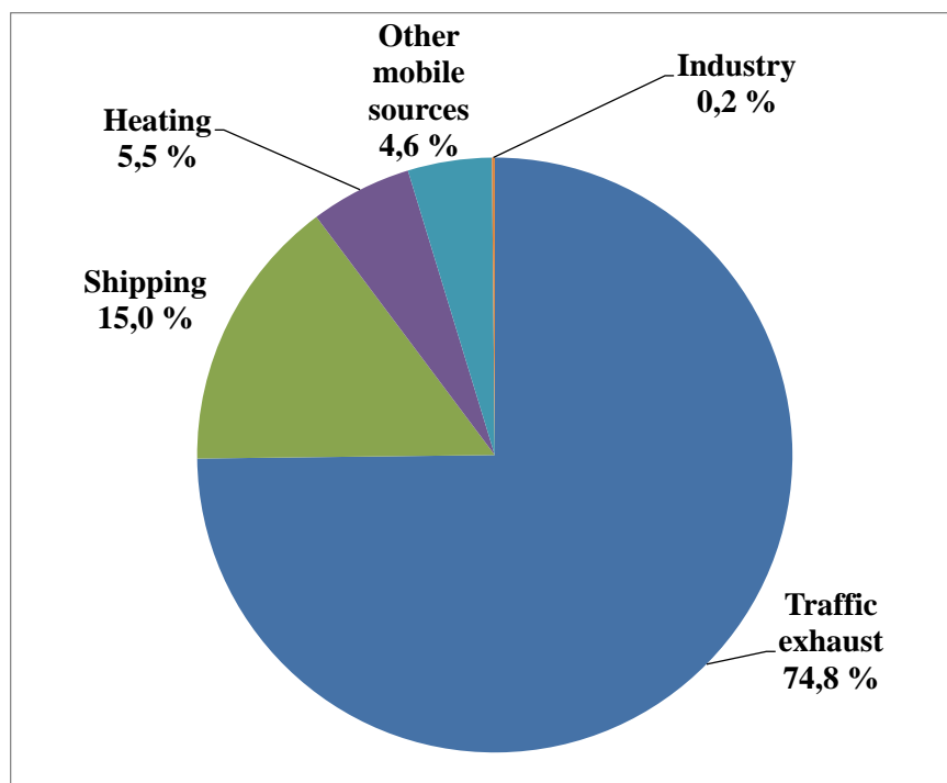
Fig. 5. The contributions of various source categories on the total emissions of particulate number in Oslo in 2008. The total amount of emissions was 1.1 \cdot 10^{24} particles/year.
