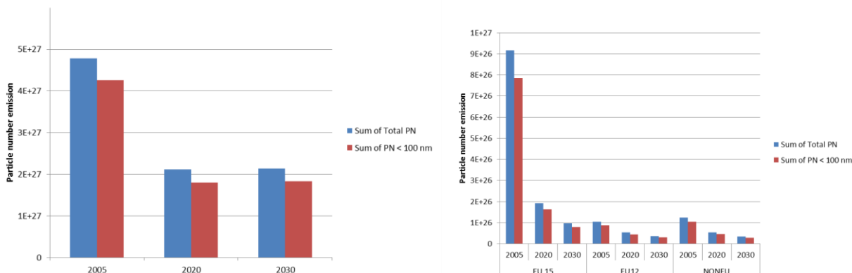
Figs. 3a-b. (a) Total anthropogenic particle number emissions and total particle number emissions in the particle size range of 10-100 nm for UNECE-Europe for 2005, 2020 and 2030 and (b) the same emissions exclusively for road transport, segmented by country group.
