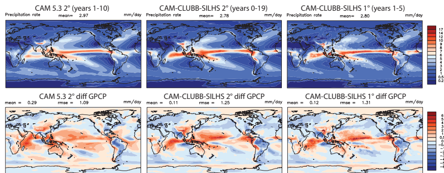
Figure 1. Total surface precipitation rate for CAM 5.3 (left), CAM-CLUBB-SILHS 2° (center), and CAM-CLUBB-SILHS 1° (right). The difference from GPCP observations of precipitation rate is shown in the second row. CAM-CLUBB-SILHS has more intense precipitation, but less of a double ITCZ than CAM 5.3.
