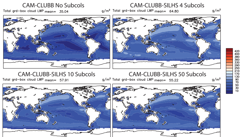
Figure 13. LWP for five years of simulation without subcolumns at all (top left), 4 subcolumns (top right), 10 subcolumns (bottom left), and 50 subcolumns (bottom right). Without subcolumns, the model has little cloud liquid water. The simulation with 4 subcolumns has a large amount of cloud liquid, which moderates in the 10 and 50 subcolumn simulations.
