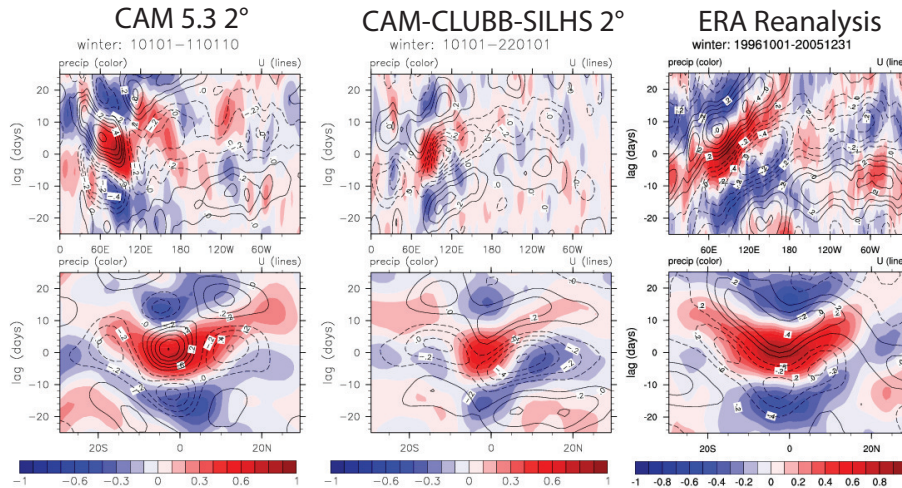
Figure 9. Lag–Longitude plots of winter MJO wave activity (top row), and Lag–Latitude plots of winter MJO wave activity (bottom row) for CAM 5.3 (left column), CAM-CLUBB-SILHS (center column), and ERA Reanalysis (right column). Precipitation is denoted by colors, zonal wind by lines. The signal in CAM-CLUBB-SILHS is weaker than observations, but the wave is moving eastward, rather than westward as in CAM 5.3.
