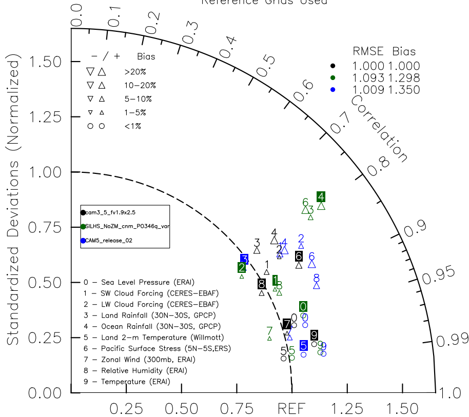
Figure 7. Taylor diagram with metrics for CAM 3.5 (black), CAM 5.3 (blue), and 2° CAM-CLUBB-SILHS (green). CAM-CLUBB-SILHS is competitive for all metrics except ocean and land rainfall, and Pacific surface stress.
