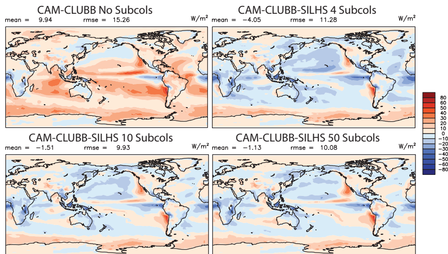
Figure 12. Simulated SWCF minus CERES-EBAF observations for five years of simulation without subcolumns at all (top left), 4 subcolumns (top right), 10 subcolumns (bottom left), and 50 subcolumns (bottom right). Without subcolumns, the clouds are too dim. The simulation with 4 subcolumns has brighter clouds than observed, and the simulations with 10 and 50 subcolumns differ little from each other.
