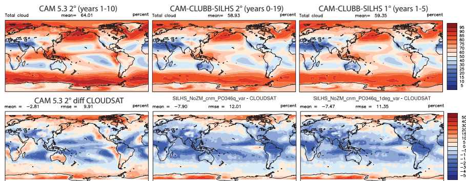
Figure 5. Total grid box cloud fraction for CAM 5.3 (left), CAM-CLUBB-SILHS 2° (center), and CAM-CLUBB-SILHS 1° (right). The difference from CLOUDSAT observations of total cloud fraction is shown in the second row. The global mean cloud fraction in CAM-CLUBB-SILHS is reduced by about 5% compared to the CAM 5.3 mean value.
