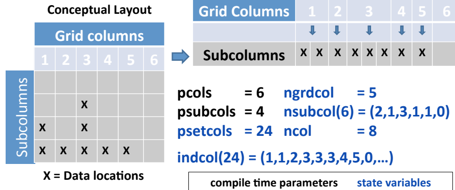
Figure A1. Schematic for CAM’s subcolumn software framework. The number of subcolumns varies by grid column, as shown in the conceptual layout (left). Internally, the subcolumns are stored in a compressed layout (right). The information on per-chunk linkages is stored in a series of software parameters, some of which can be set by the user (black) and others of which are internally calculated (blue). pcols is the maximum number of grid columns, psubcols is the maximum number of subcolumns, psetcols is the maximum number of all columns (= pcols · psubcols ), ngrdcol is the actual number of grid columns that contain data, nsubcol ( pcols ) is the number of subcolumns in each grid column with data, ncol is the total number of all subcolumns with data, and indcol ( psetcols ) is the grid index for each subcolumn, which is used for mapping subcolumns back to grid columns.
