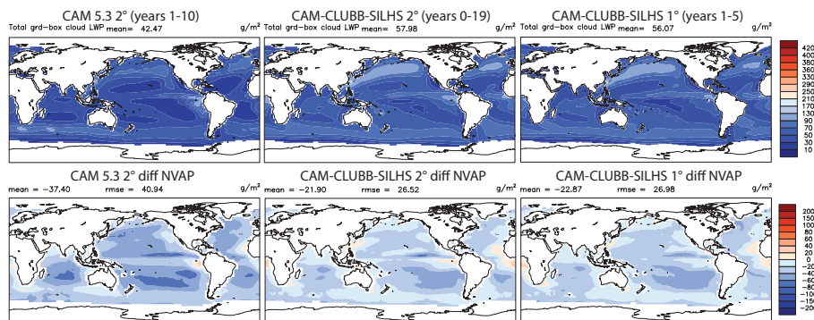
Figure 6. Total grid box liquid water path (LWP) for CAM 5.3 (left), CAM-CLUBB-SILHS 2° (center), and CAM-CLUBB-SILHS 1° (right). The difference from NVAP observations of LWP is shown in the second row. The global mean LWP in CAM-CLUBB-SILHS is about 35 % higher than that of CAM 5.3.
