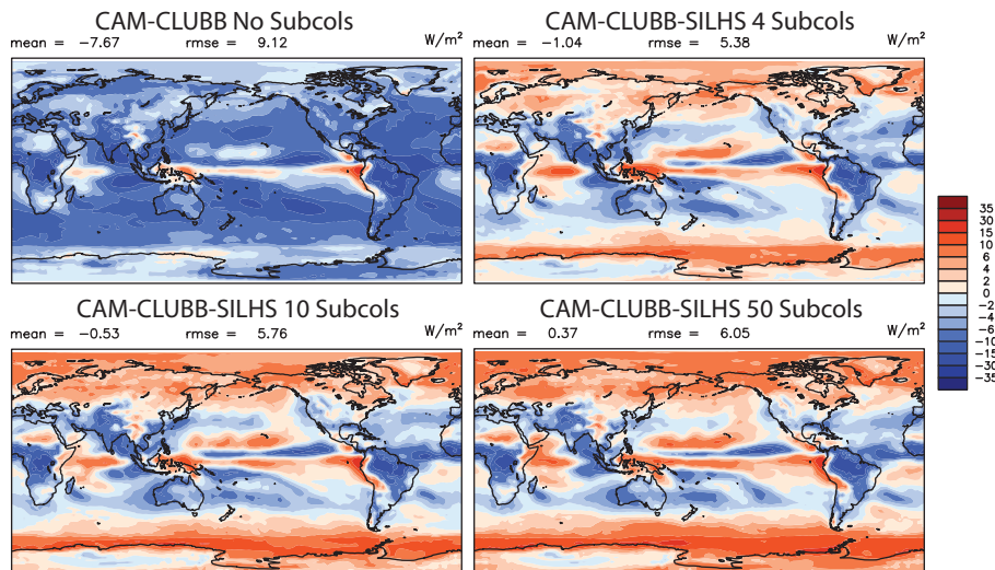
Figure 11. LWCF difference from CERES-EBAF observations for five years of simulation without subcolumns at all (top left), 4 subcolumns (top right), 10 subcolumns (bottom left), and 50 subcolumns (bottom right). Without subcolumns, the LWCF has a severe low bias. The simulation with 4 subcolumns has the lowest global error, and very little changes between the simulations with 10 and 50 subcolumns.
