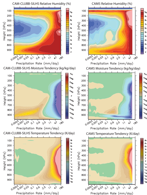
Figure 10. Daily average profiles of fields per daily average value of precipitation for the region between latitudes 15^{\circ} N and 15^{\circ} S and longitudes 60 to 180^{\circ} E over one year. Relative humidity for CAM-CLUBB-SILHS (top left) and CAM5 (top right), total physics moisture tendencies for CAM-CLUBB-SILHS (middle left) and CAM5 (middle right), and total physics temperature tendencies for CAM-CLUBB-SILHS (bottom left) and CAM5 (bottom right) are shown. Because CAM-CLUBB-SILHS is a unified parameterization, there is a smoother transition from light to intense precipitation values for all fields.
