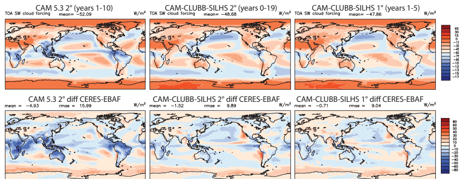
Figure 4. Top of the atmosphere short wave cloud forcing (SWCF) for CAM 5.3 (left), CAM-CLUBB-SILHS 2° (center), and CAM-CLUBB-SILHS 1° (right). The difference from CERES-EBAF observations of SWCF is shown in the second row. CAM-CLUBB-SILHS reduces the SWCF low bias over tropical land regions seen in CAM 5.3.
