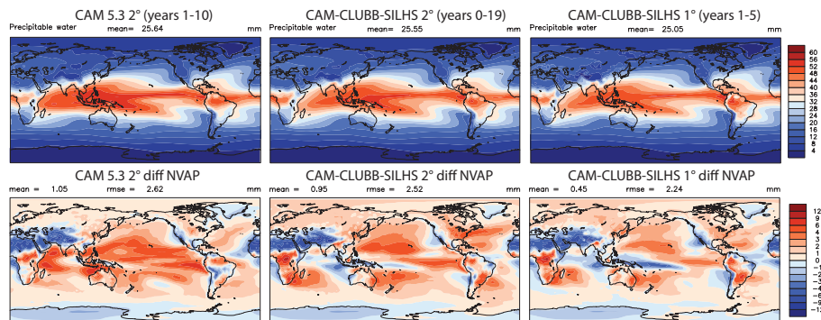
Figure 2. Total column water vapor field for CAM 5.3 (left), CAM-CLUBB-SILHS 2° (center), and CAM-CLUBB-SILHS 1° (right). The difference from National Aeronautics and Space Administration (NASA) Water Vapor Project (NVAP) satellite observations (model – obs) is shown in the second row. CAM-CLUBB-SILHS reduces the overall moist bias seen in CAM 5.3.
