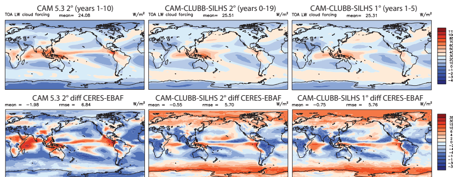
Figure 3. Top of the atmosphere long wave cloud forcing (LWCF) for CAM 5.3 (left), CAM-CLUBB-SILHS 2° (center), and CAM-CLUBB-SILHS 1° (right). The difference from Clouds and Earth's Radiant Energy Systems (CERES) Energy Balanced and Filled (EBAF) observations of LWCF (model – obs) is shown in the second row. CAM-CLUBB-SILHS has a slightly lower global error in LWCF than CAM 5.3 due to an increase in cloud forcing in the mid-latitudes and polar regions.
