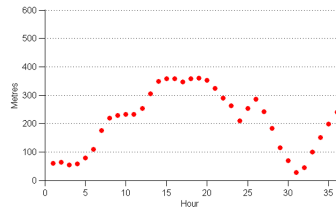
(c) Point, 10m current
