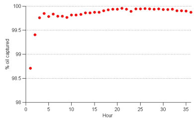
(e) Point, 30m current
