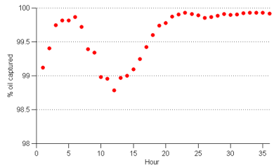
(a) Point, 0m current
