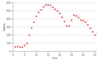
(a) Point, 0m current
