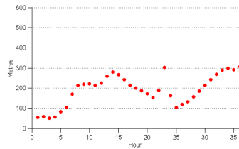
(e) Point, 30m current
