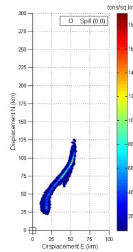
(b) MEDSLIK, hr 300, 10m current
