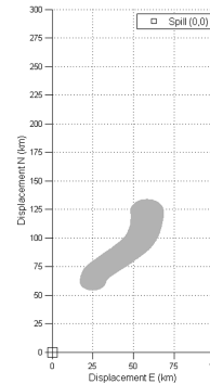
(f) CranSLIK, hr 400, 30m current
