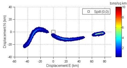
(c) MEDSLIK, 10m current
