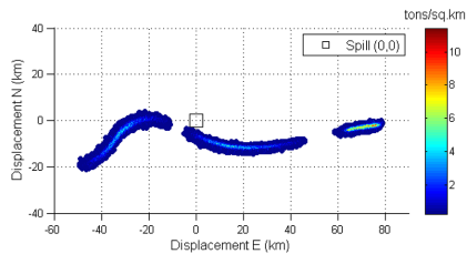
(e) MEDSLIK, 30m current
