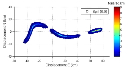
(a) MEDSLIK, 0m current
