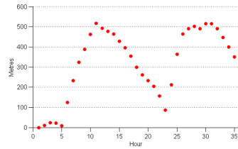
(b) Contour, 0m current
