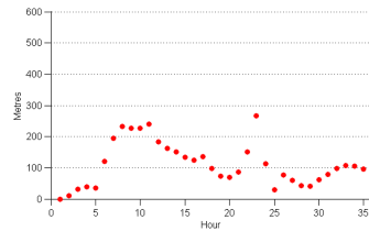
(f) Contour, 30m current
