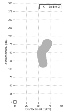
(e) CranSLIK, hr 467, 10m current
