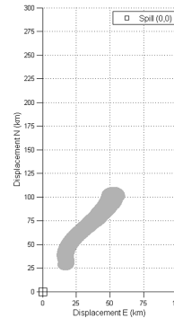
(e) CranSLIK, hr 300, 10m current
