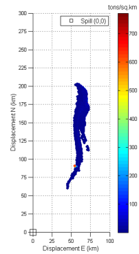
(b) MEDSLIK, hr 467, 10m current
