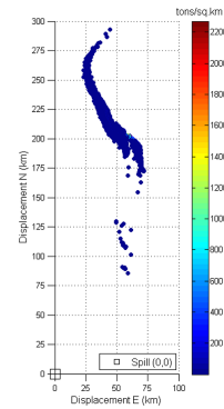
(c) MEDSLIK, hr 600, 30m current
