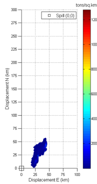
(a) MEDSLIK, hr 240, 0m current
