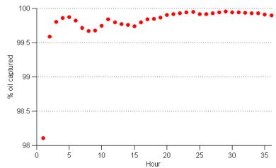
(c) Point, 10m current
