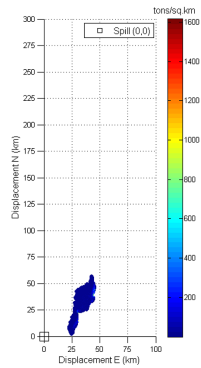
(a) MEDSLIK, hr 277, 0m current
