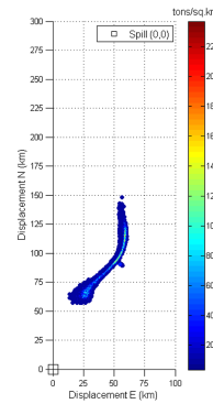
(c) MEDSLIK, hr 400, 30m current
