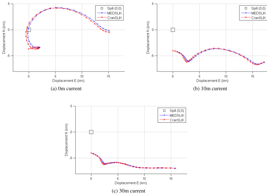
Figure 3. Centre of mass trajectory forecasts (hours 1–36) for the the Algeria-contour case using the current at different depths as the advective current.
