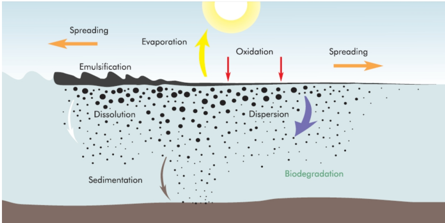
Figure 1. Weathering process, from ITOPF (2014a).
