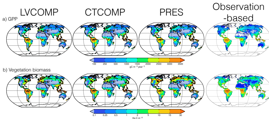
Figure 7. Geographical distribution of modelled GPP (a), and vegetation biomass (b) from simulations that use dynamically modelled fractional coverages of PFTs based on the original LV equations (LVCOMP, leftmost column), and the modified LV equations (CTCOMP, second column). The third column shows simulation results that use prescribed PFT fractional cover based on the modified Wang et al. (2006) dataset (PRES). The observation-based dataset in the fourth column for GPP is from Beer et al. (2010) and for vegetation biomass it is from Ruesch and Holly (2008).
