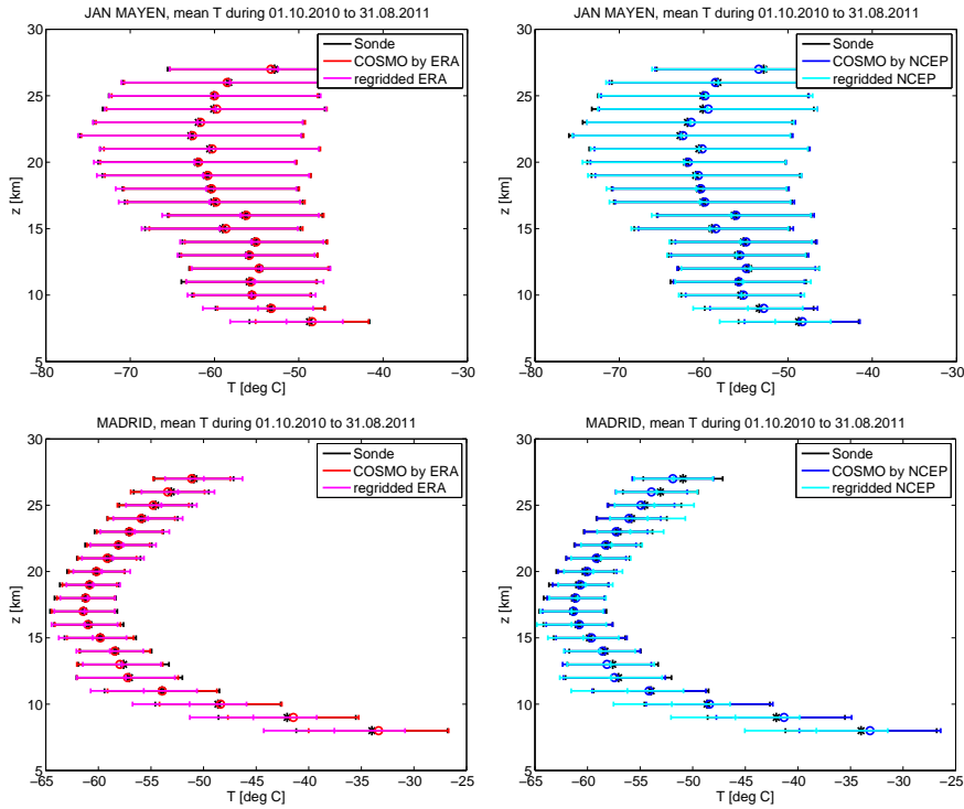
Figure 6. Mean temperature values at each height for the station on Jan Mayen, station no. 20, on the top, and for Madrid, station no. 1, on the bottom, showing results of the run forced by ERA-Interim (left) and NCEP (right). The horizontal lines give the 1\sigma standard deviation.
