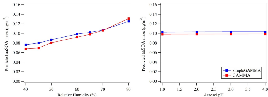
Figure 4. Comparison of predicted aaSOA after 12 h of simulated time with respect to RH at pH 1 (left) and with respect to pH at 65 % RH (right), high-NO x conditions.
