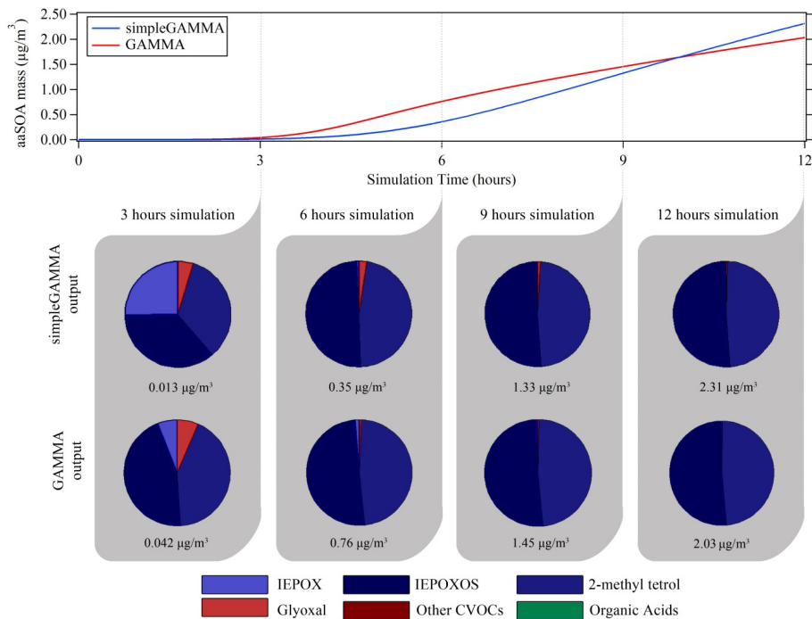
Figure 1. Comparison of simpleGAMMA and GAMMA under low-NO x conditions, pH1, RH 65%.
