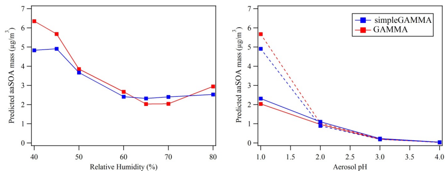
Figure 2. Comparison of predicted aaSOA after 12 h of simulated time as a function of RH at pH 1 (left) and pH at 45 and 65 % RH (right, dotted and solid lines respectively), low- \text{NO}_x conditions.
