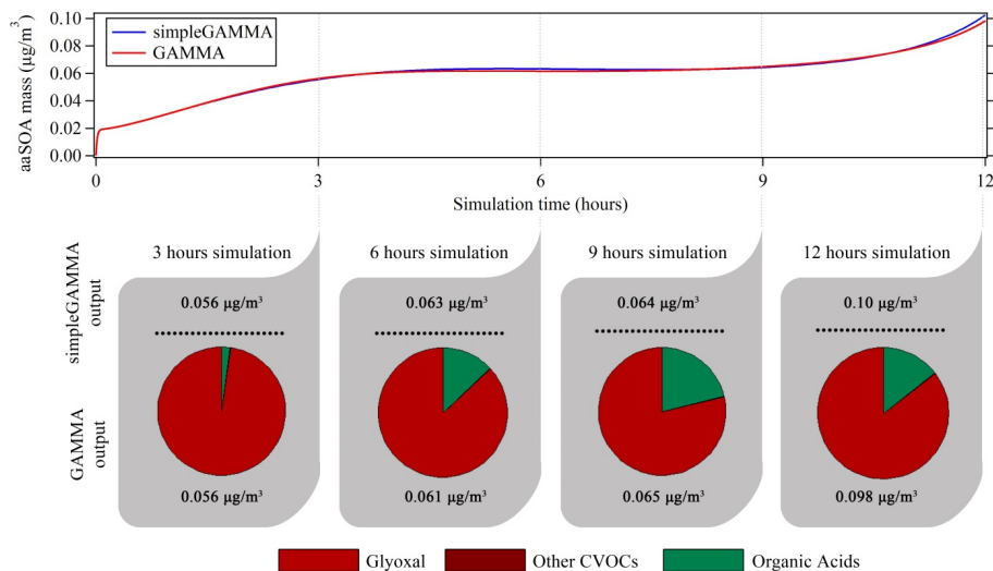
Figure 3. Comparison of high-NO x simpleGAMMA and high-NO x GAMMA, pH1, RH65.
