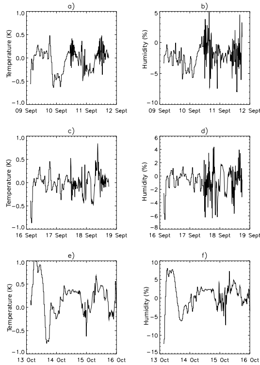
Figure 5: Difference between shorter IOP simulations and the longer term simulation (IOP minus long term simulation) for screen temperature (a,c,e) and relative percentage differences in screen-level specific humidity (b,d,f) at Duffryn for IOPs 4-5 (a,b), IOPs 6-7 (c,d), IOPs 8-9 (e,f).
