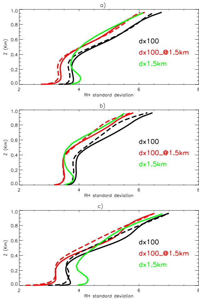
Figure 14: Standard deviations of relative humidity values simulated in, \Delta 100\text{m} output (black), \Delta 100\text{m} output averaged to 1.5\text{km} resolution (red) and \Delta 1.5\text{km} output (green). Solid lines are simulations with \text{RH}_{\text{crit}} profiles from the operational 1.5\text{km} model, while dashed lines correspond to the \text{RH}_{\text{crit}} profile with higher thresholds described in Vosper et al. (2013a). The subfigures show (a) total mean profiles, (b) average day profiles (07-19 UTC) and (c) night profiles (19-07 UTC).
