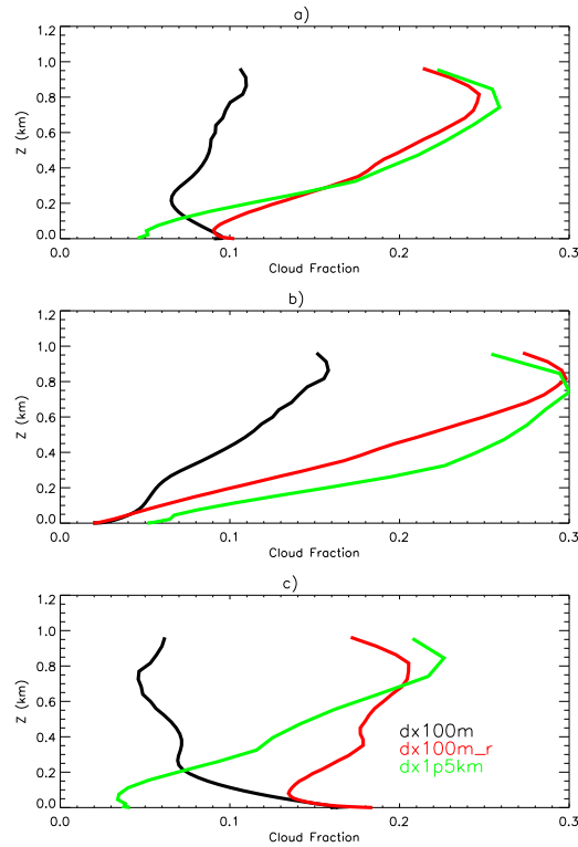
Figure 11: The mean cloud cover profile for the lowest kilometre for a) all hours, b) 07-19 UTC and c) 19-07 UTC, averaged over all days in the re-run period (15-25 September).
