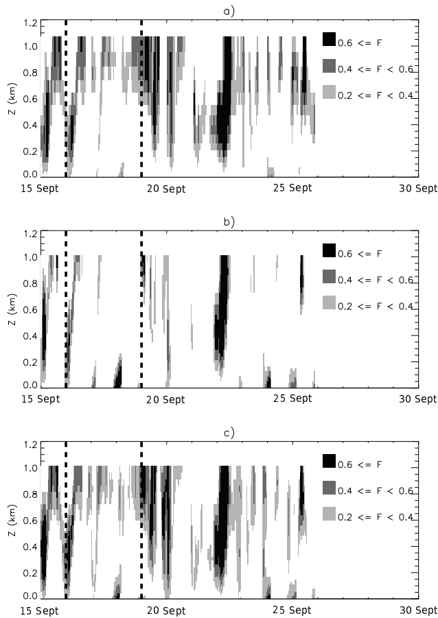
Figure 10: Hourly area averaged profiles of model cloud fraction ( F ) for a) \Delta 1.5\text{km} , b) \Delta 100\text{m} and c) \Delta 100\text{m}_r . Vertical lines show 00 UTC 16 September and 00 UTC 19 September, and correspond to the period shown in figure 13. Area averaged are calculated over the 10km by 10km domain illustrated in figure 1.
