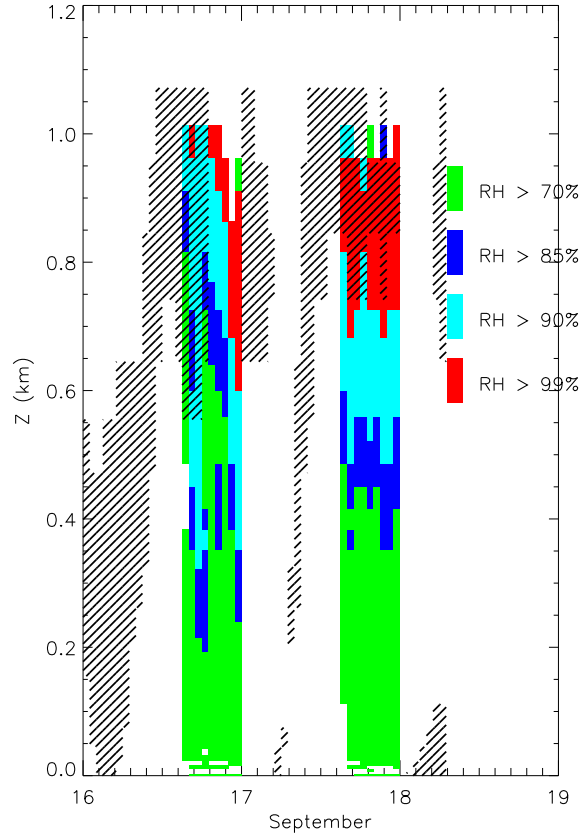
Figure 13: Radiosonde relative humidity profiles at Spring Hill during 16-18 September. Also shown are \Delta 1.5\text{km} cloud fractions above 20% (diagonal hatching).
