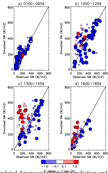
Figure 9: Bias in \Delta 100\text{m} simulated downward shortwave radiation and its relationship to bias in the screen level temperature, at Spring Hill. The temperature bias is represented as the colour and size of the marker (simulated - observed).
