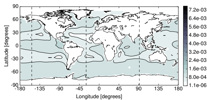
Figure 29. N-DOP model: Difference between the phosphate concentration of the spin-up and the Newton solution at the first layer (0 – 50 m) in the Euclidean norm. Units are mmol P m -3 .
