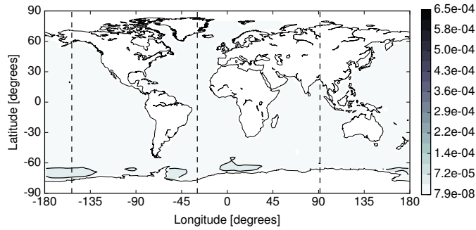
Figure 214. NPZ-DOP model: Difference between the phosphate concentration of the spin-up and the Newton solution at the first layer (0 – 50 m) in the Euclidean norm. Units are \text{mmol P m}^{-3} .
