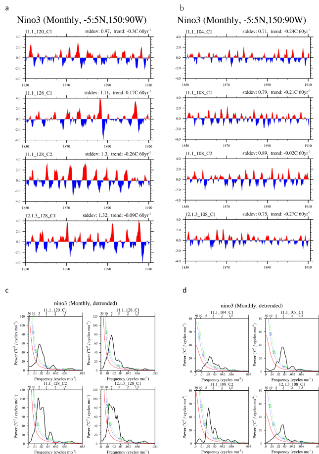
Figure 4. ENSO characteristics. (a–b) Time series of Niño-3 index ( 5^{\circ}\text{S} – 5^{\circ}\text{N} , 150 – 90^{\circ}\text{W} ) from the first four simulations of CESM1 and FGOALS-g2, respectively. (c–d) : Power spectrum of Niño-3 index, corresponding to (a–b) .
