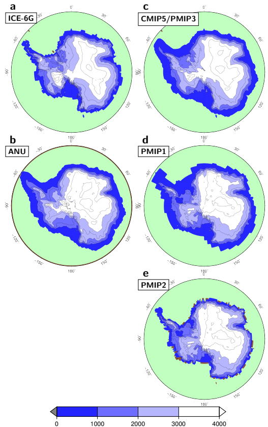
Figure 3. Surface elevation (m) of Antarctica at the LGM from the (a) ICE-6Gv.2, (b) ANU reconstructions, and for (c) the CMIP5/PMIP3 composite compared to the ice sheets used in (d) PMIP1 and (e) PMIP2. The GLAC-1a reconstruction for Antarctica is identical to that of ICE-6G, and is therefore not shown.
