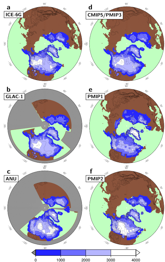
Figure 1. Surface elevation (m) at the Last Glacial Maximum (LGM) Northern Hemisphere ice sheets from the (a) ICE-6Gv.2, (b) GLAC-1a and (c) ANU reconstructions, and for (d) the CMIP5/PMIP3 composite compared to the ice sheets used in (e) PMIP1 and (f) PMIP2.
