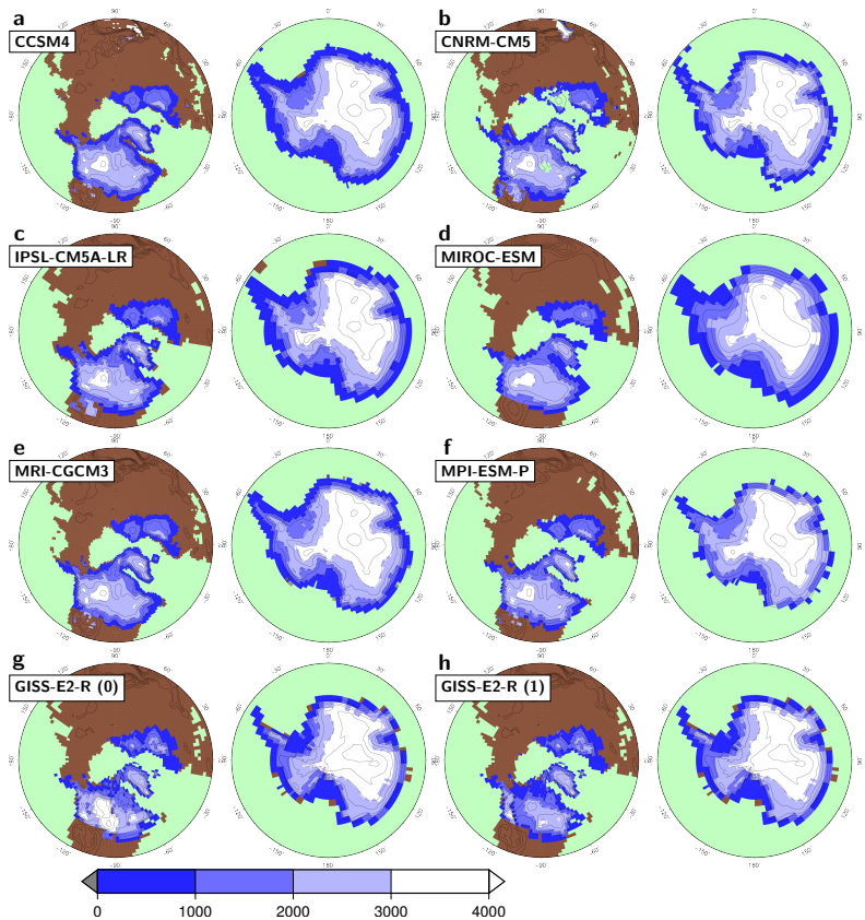
Figure 9. Implementation of the CMIP5/PMIP3 composite ice sheet in individual models. These plots show that there are small differences in prescribed ice sheet between models because of differences in e.g. model type and resolution.
