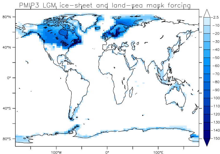
Figure 6. Estimation of the difference in radiative forcing and feedbacks at the LGM compared with pre-industrial conditions caused by imposition of the CMIP5/PMIP3 ice sheet and the change in the land-sea mask. The map is a composite of the results from five ocean-atmosphere models showing the spatial patterns of the change in total forcing associated with the expanded Northern Hemisphere ice sheets at the LGM and with the increase of land area due to lowered sea level.
