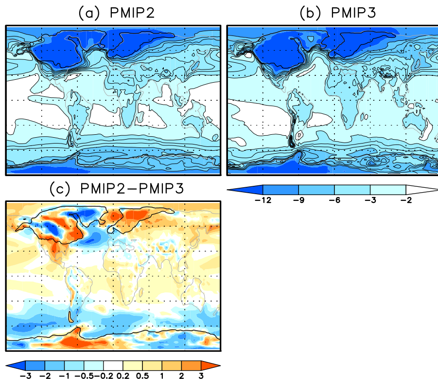
Figure 8. Change in mean annual temperature (MAT) in the (a) PMIP2 and (b) CMIP5/PMIP3 coupled ocean-atmosphere simulations. Each of these plots is an ensemble average of all the LGM simulations in PMIP2 and CMIP5/PMIP3 respectively. The difference between the ensemble mean results for the two generations of experiments is shown in plot (c). The land and ice masks are the same as Fig. 7. Contour lines are also illustrated in (a, b). The contour interval is 1^{\circ}\text{C} where the temperature is higher than -9^{\circ}\text{C} .
