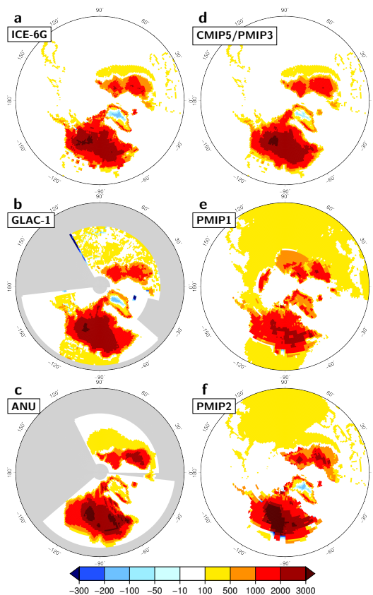
Figure 2. Difference in surface elevation (m) of the Northern Hemisphere ice sheets at the LGM compared to the present-day from the (a) ICE-6Gv.2, (b) GLAC-1a and (c) ANU reconstructions, and for (d) the CMIP5/PMIP3 composite compared to the ice sheets used in (e) PMIP1 and (f) PMIP2. The region shown is between 40 and 90° N .
